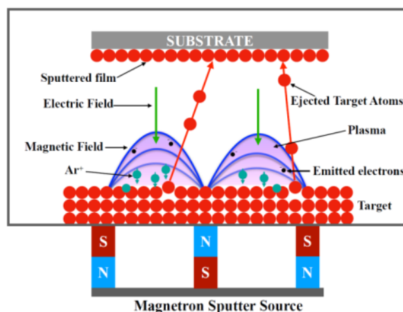
Figure 2-1 Schematic of magnetron sputtering process. Extracted from [89].
