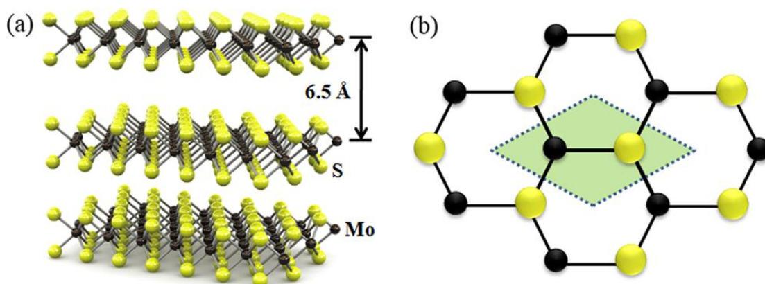
Figure 1. 6 The crystal structure of \text{MoS}_2 .
