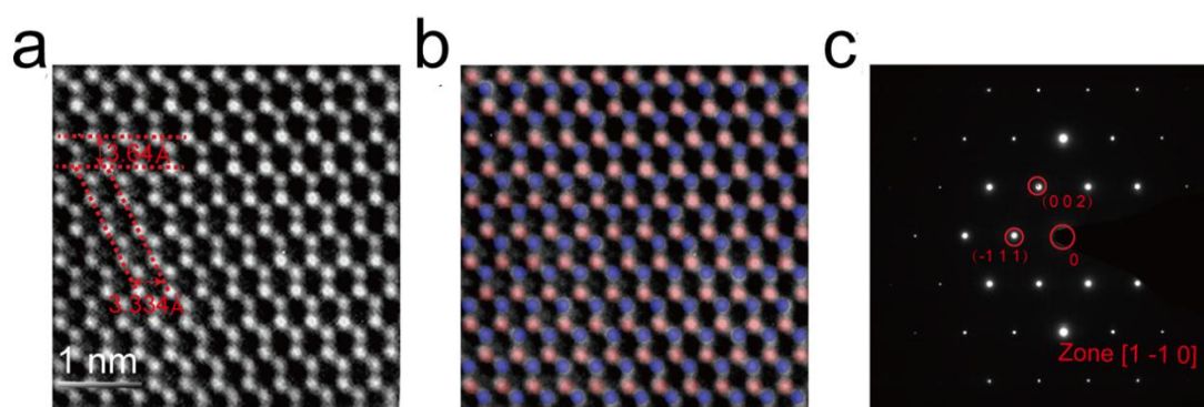
Figure 4.3 Structure characterization.
