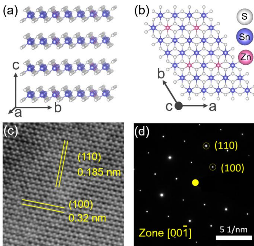
Figure 5. 4 Crystal structure.
