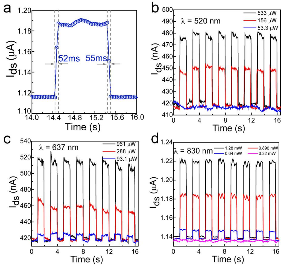
Figure 4. 12 Optoelectronic properties of the GeAs based device.
