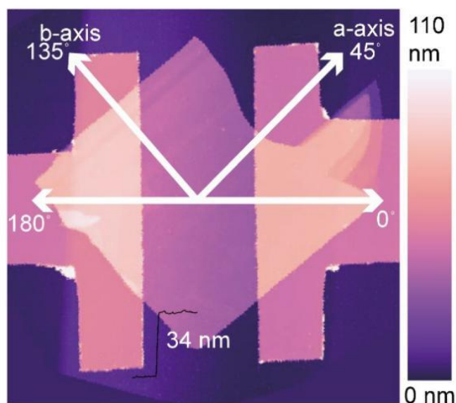
Figure 4. 11 Atomic force microscope image of the device based on GeAs nanosheets.
