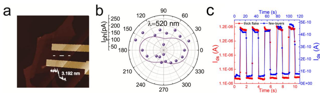
Figure 4. 18 Photo response of thin GeAs based device. (a) AFM image of the few-layer GeAs device. (b) Experimental polarized photocurrent under the linear-polarization laser of 520 nm. (c) Time dependent I_{ds} of thick flake GeAs and few-layers GeAs under the zero V_{ds} and 520 nm laser of 541 \mu\text{W} power.
