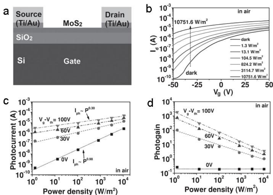
Figure 1. 8 The photodetector based on ML \text{MoS}_2 .
