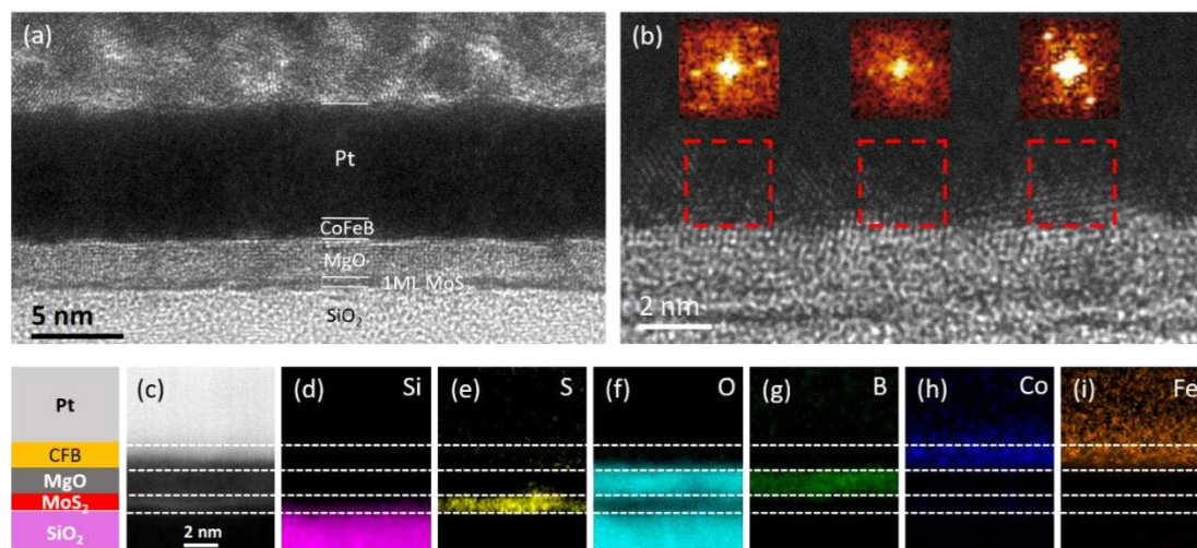
Figure 3. 11 Interfacial structure and chemical characterization of MoS 2 /MgO/CoFeB/Pt heterostructure.
