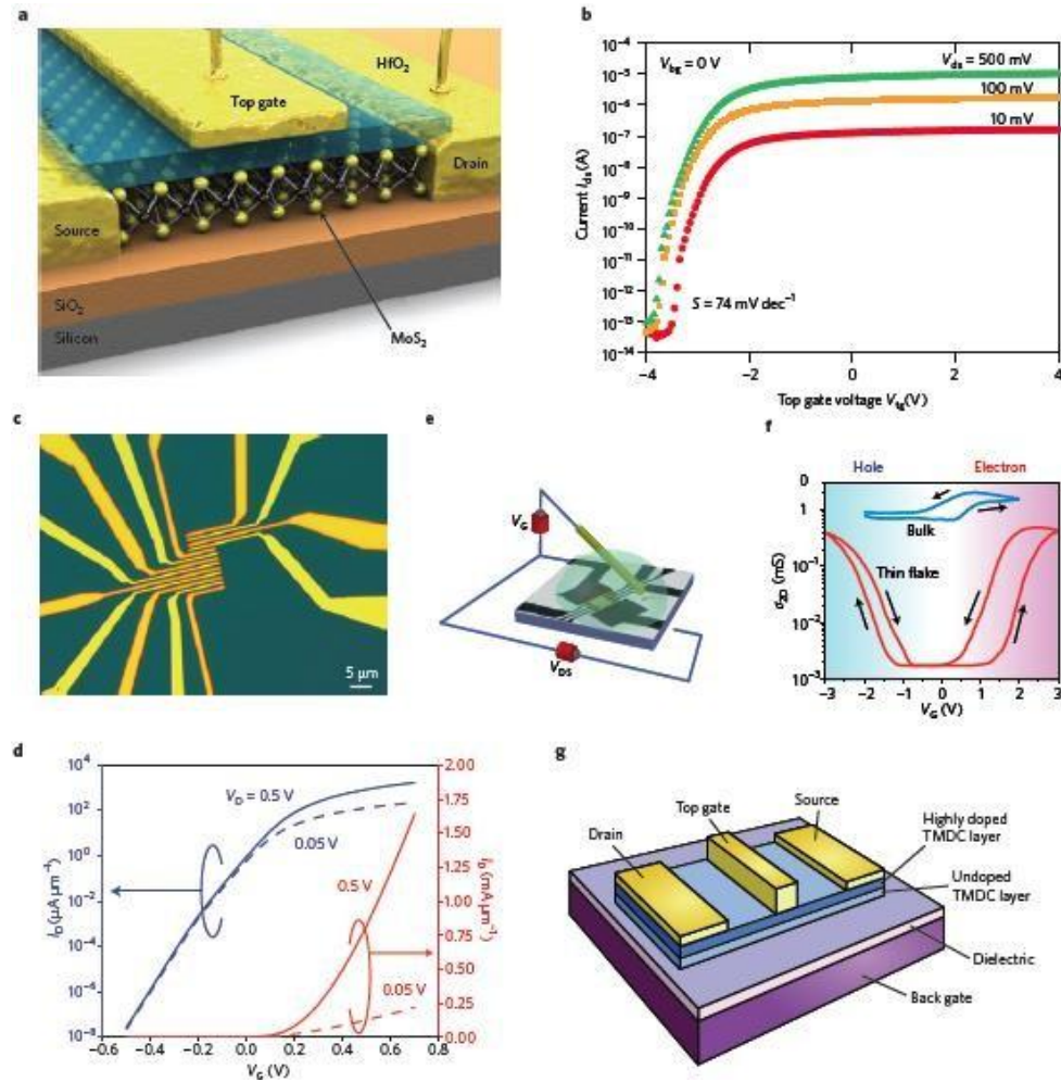
Figure 1. 7 MoS 2 based electrical devices.
