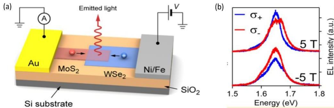
Figure 1.15: (a) Diagram of the device. Under the application of a positive bias voltage to the Ni / Fe permalloy electrode, holes are injected from the permalloy electrode and recombine in the junction with the electrons injected from the side of the MoS 2 , which causes light emission. (b) Electroluminescence spectra of a spin valley LED for different values of magnetic fields, acquired for polarizations ( \sigma^+ ) and ( \sigma^- )[39].
