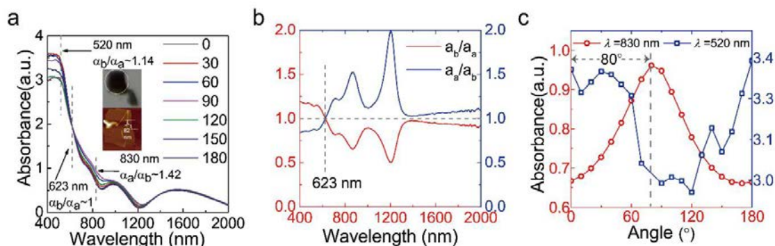
Figure 4. 10 Polarization-resolved absorption spectra. (a) Polarization-resolved absorption spectra in experimental with the spectral range from 400 to 2000 nm in steps of 30°. The microscope image and AFM image of GeAs are inset. (b) The dichroism ratios a_b/a_a (red line) and a_a/a_b (blue line) are extracted from (a). (c) Absorption intensity as a function of angle varies under 520 nm (blue plots and line) and 830 nm (red plots and line), respectively
