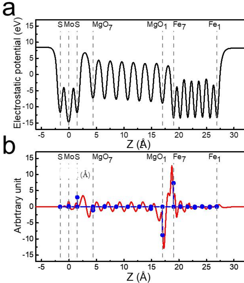
Figure 3. 16 (a) z-variations of the xy-averaged electrostatic part of the potential energy. (b)
