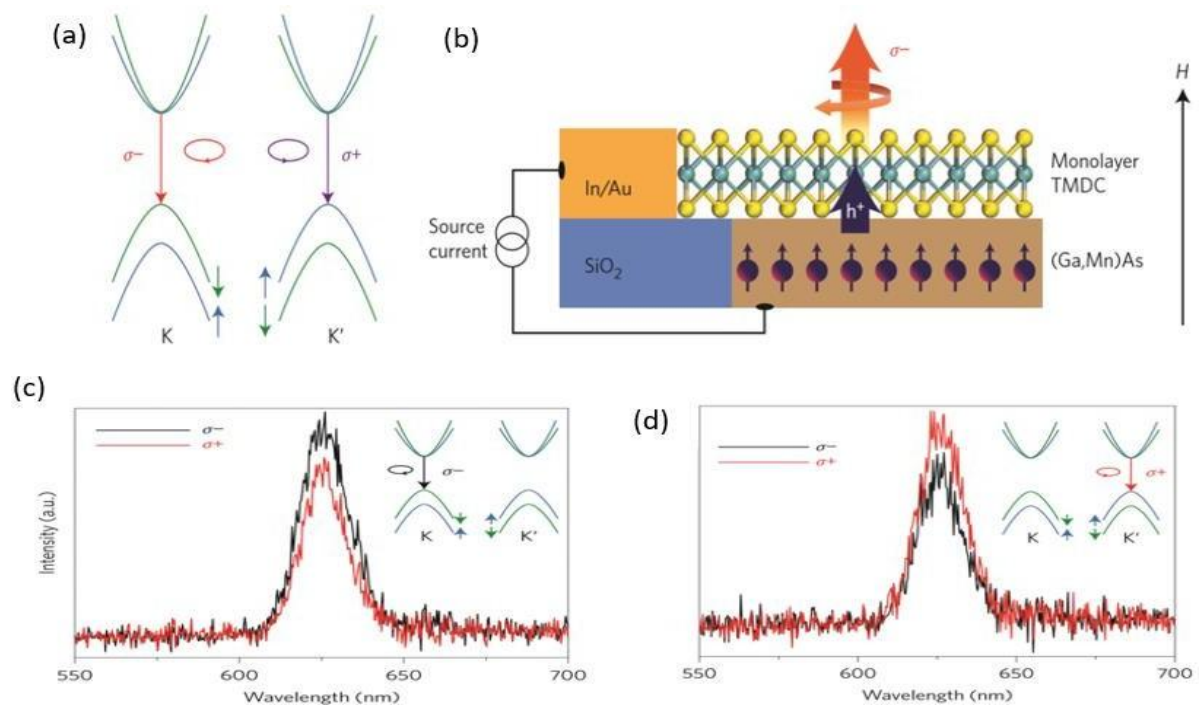
Figure 1. 14: (a) Electronic structure in the K and K 'valleys of the TMDCs monolayer. (b) Schematic of the single-layer TMDCs / (Ga, Mn) As device used for the electrical polarization of valleys. (c) Electroluminescence spectra polarized under an external magnetic field of 400 Oe perpendicular to the surface with a current of 15 \mu A. (d) Electroluminescence spectra polarized under an external magnetic field of 400 Oe perpendicular to the surface but inverted from (c).[38]
