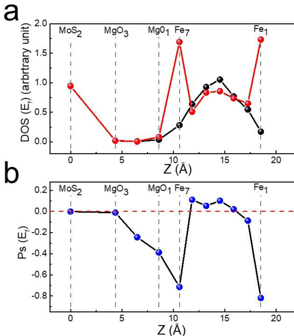
Figure 3. 20 (a) z-dependence of the DOS at the Fermi level, calculated for majority and minority spin electrons. (b) Profile of spin polarization calculated from the spin-resolved DOS.
