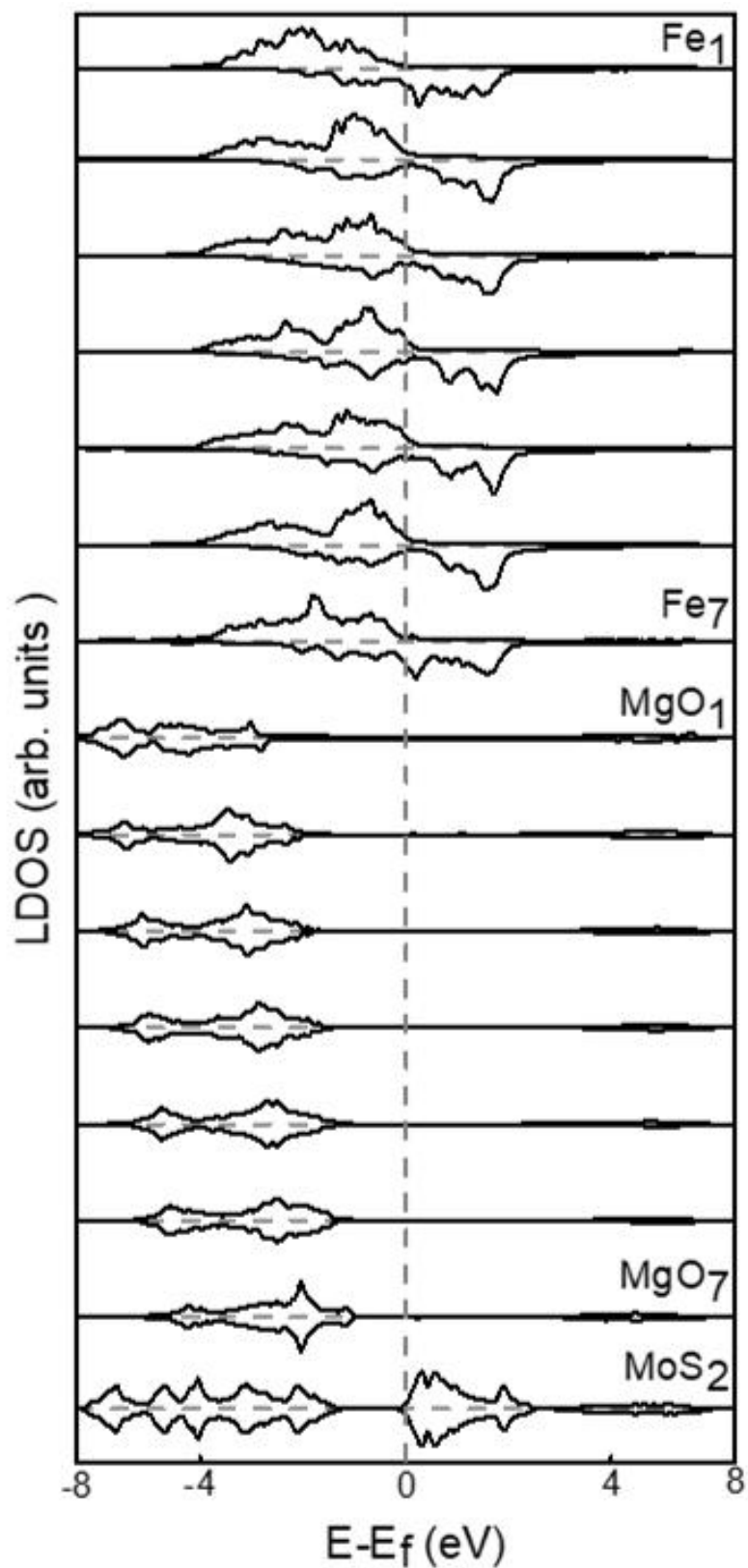
Figure 3. 15 Integrated majority and minority DOS over atomic spheres belonging to the successive atomic layers of the supercell.
