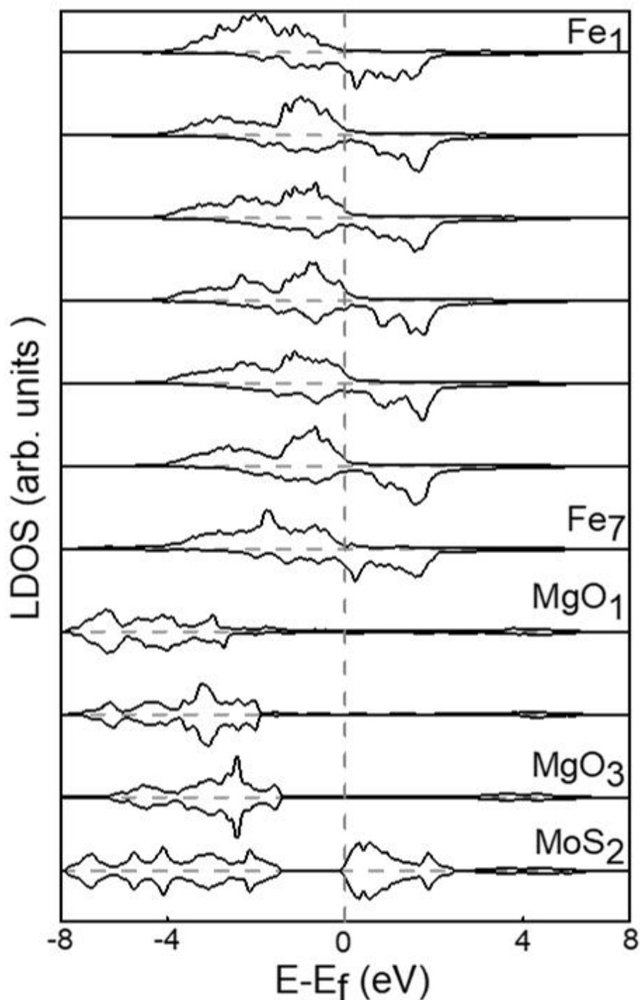
Figure 3. 18 Integrated majority and minority DOS over atomic spheres belonging to the successive atomic layers of the supercell.
