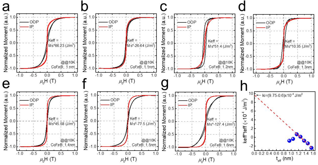
Figure 3. 6 (a-g) Out-of-plane and in-plane M-H curves for samples with different CoFeB thicknesses with T_{an}=250^\circ\text{C} measured at 10K. (a) 1nm, (b) 1.1nm, (c) 1.2nm, (d) 1.3nm, (e) 1.4nm, (f) 1.5nm, (g) 1.6nm. (h) t_{eff} dependence of the product of K_{eff} and t_{eff} , where the intercept to the vertical axis of the linear extrapolation corresponds to interface anisotropy
