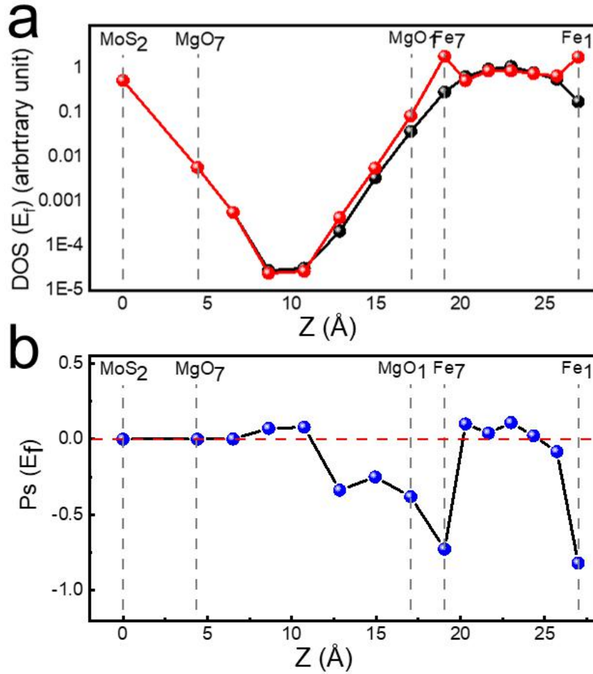
Figure 3. 17 (a) z-dependence of the DOS at the Fermi level, calculated for majority and minority spin electrons. (b) Profile of spin polarization calculated from the spin-resolved DOS.
