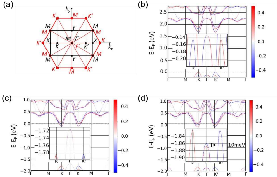
Figure 3. 21 Band structure of the MoS 2 ML in the multilayer structure. (a) Brillouin zone of the unit cells. The red lines represent the hexagonal Brillouin zone of the primitive unit cell of the MoS 2 ML. The black lines represent the rectangular Brillouin zone of the multilayer structure. (b) Band structure of monolayer MoS 2 calculated with a conventional rectangular unit cell. Inset: Magnified valence band structures. (c, d) Contribution of the MoS 2 layer to the band structure of the multilayer with (c) 7 MLs of MgO and (d) 3 MLs of MgO. The red and blue lines respectively show the positive and negative values of the spin projection s_z (in units of \hbar ). Insets: Magnified valence band structures show a negligible Zeeman splitting for 7 MLs of MgO but a large splitting of 10meV at \Gamma point for 3 MLs of MgO.
