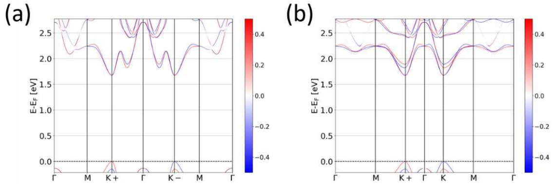
Figure 3. 22 (a) Band structure of monolayer MoS 2 defined in a hexagonal lattice. (b) Band structure of monolayer MoS 2 defined in a rectangular lattice.
