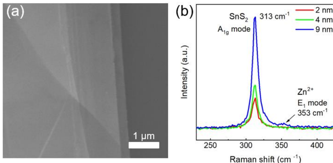
Figure 5. 2 Raman spectrum.
