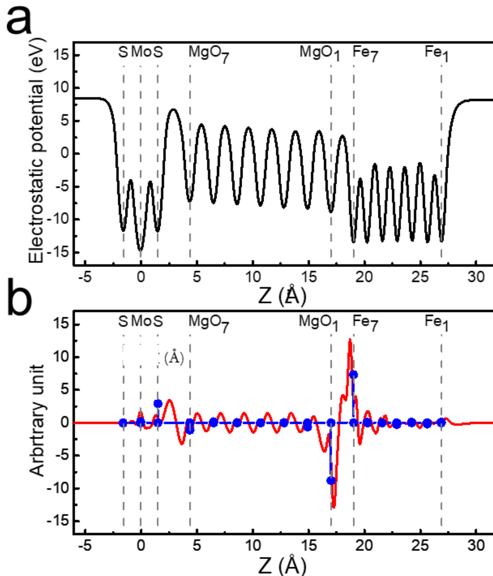
Figure 3. 15 (a) z-variations of the xy-averaged electrostatic part of the potential energy. (b)
