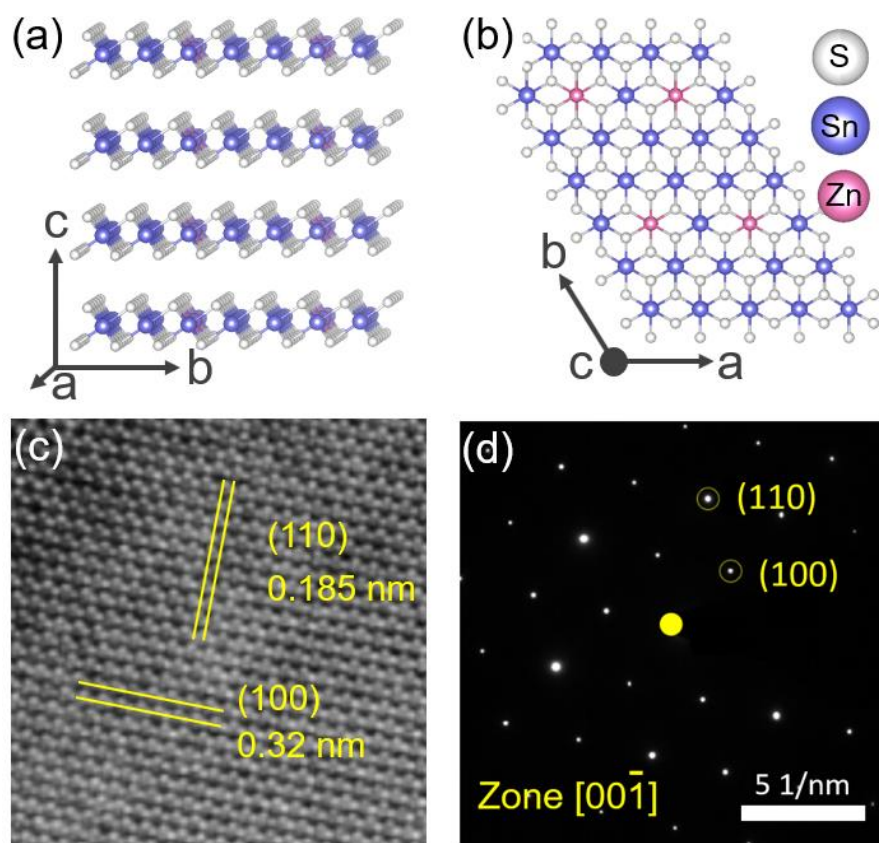
Figure 5. 4 Crystal structure.
