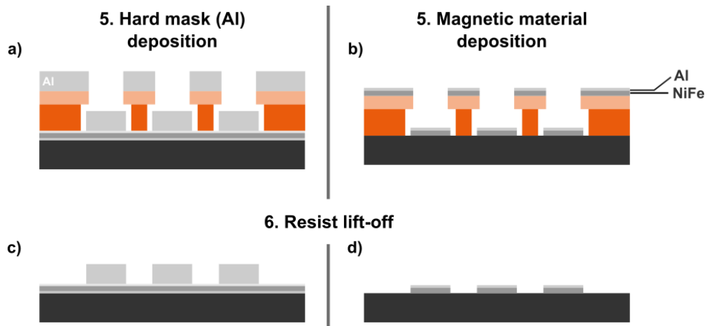
Fig.2-3: a) Deposition by e -beam evaporation of 100 nm-thick Al layer acting as hard mask in order to perform IBE and b) NiFe(20)/Al(3) also by evaporation for the lift-off process; c)-d) result of lift-off of the remaining resist and surplus of material by Remover1165 hot bath and sonication.
