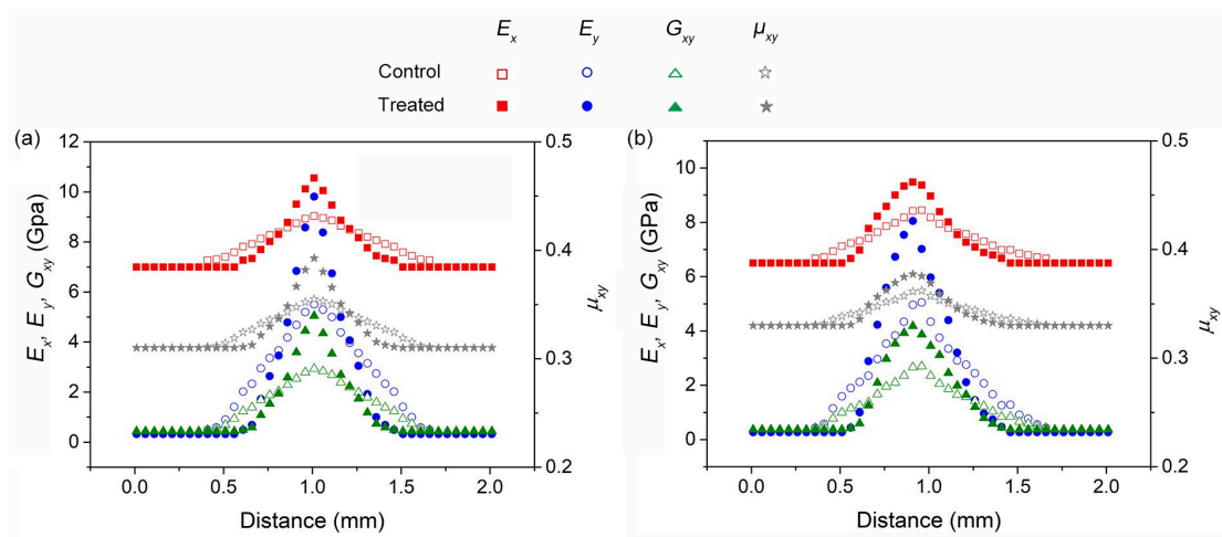
Fig.5-4 Elastic constants distribution for (a) masson pine and (b) poplar single bonding interphase in 5-ply laminated-wood before and after HVEF treatment.
