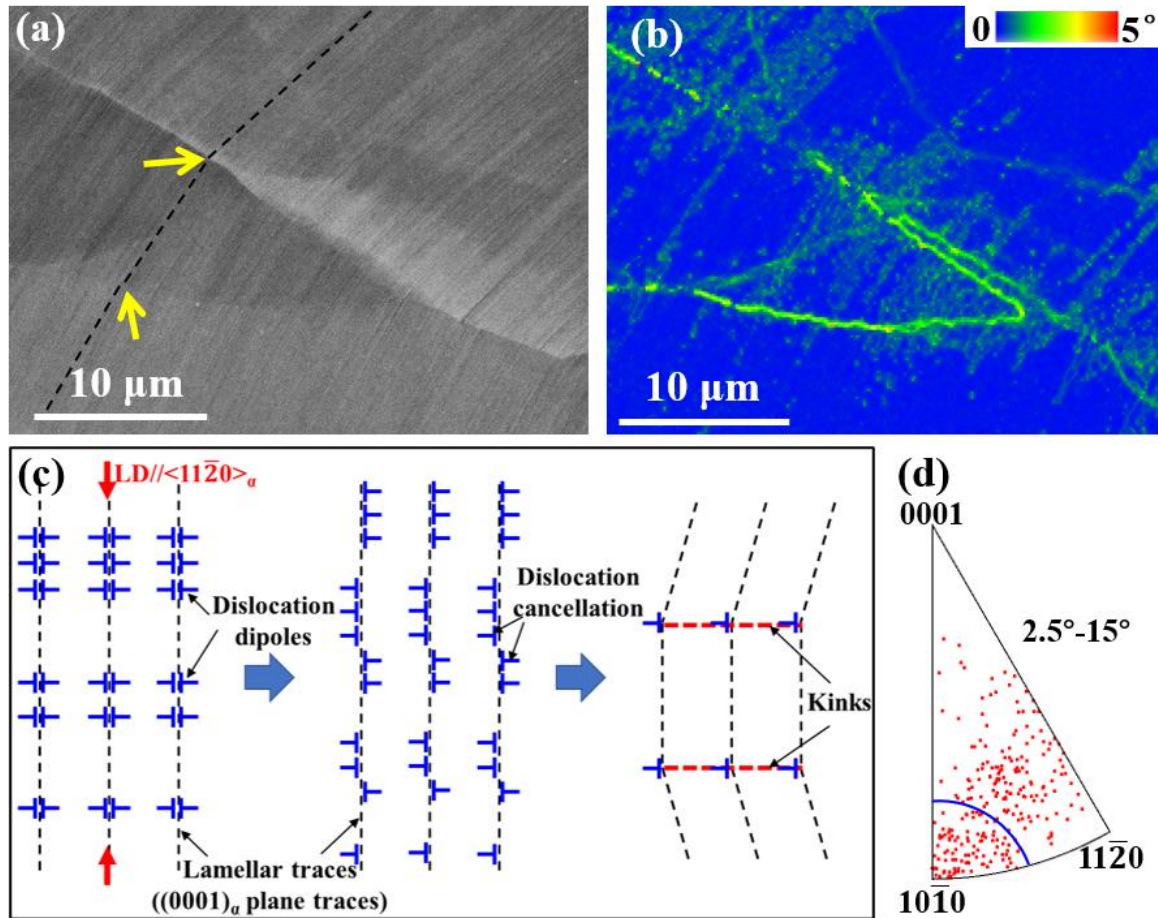
Fig. 4-9 (a) SEM-BSE micrograph of the magnified local areas outlined with red rectangle in G5 oriented with nearly \langle 11\bar{2}0 \rangle_{\alpha} //LD in Fig. 4-5 (a); (b) Kernel Average Misorientation (KAM) micrograph; (c) Schematic diagram illustrating the formation of kinks; (d) Disorientation axis projection.
