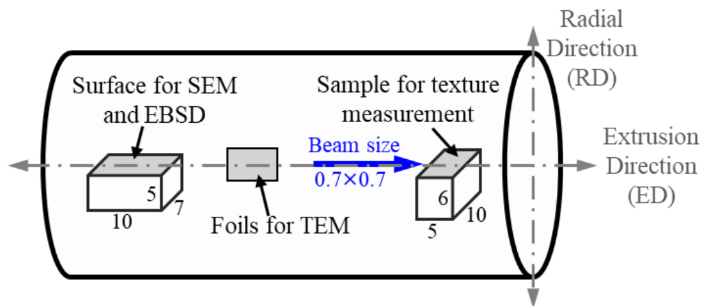
Fig. 5-1 Positions of the samples for microstructural observation and texture measurement in the extruded rod. The extrusion direction (ED) and radial direction (RD) constitute the coordinate system of samples for texture measurement and EBSD observation. Dimensions indicated in the figure are in mm.
