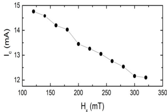
Figure 4.3 The critical current density for SOT switching with 100 μs pulses is inversely proportional to the in-plane H_x field, as reported previously 90
