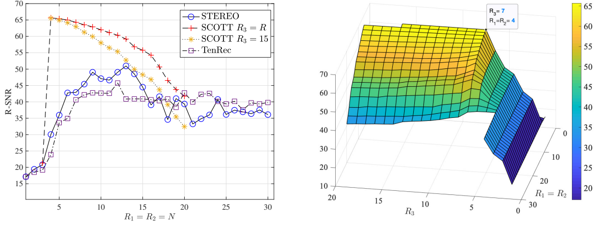
Figure 2.10: R-SNR as a function of the ranks.
