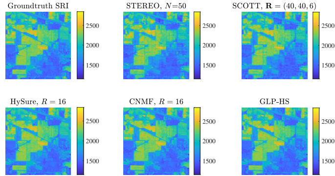
Figure 2.3: Spectral slice no.120 of the SRI, Indian Pines.
