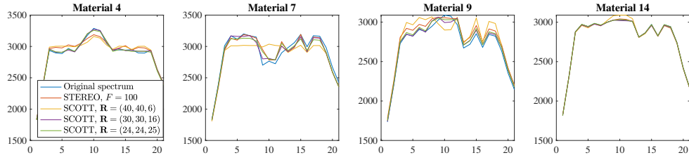
Figure 2.22: Spectral signatures at spectral bins no.80 to 100.
