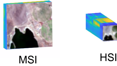
Figure 1.2: HSI and MSI of a same scene above Lake Tahoe, Nevada.
