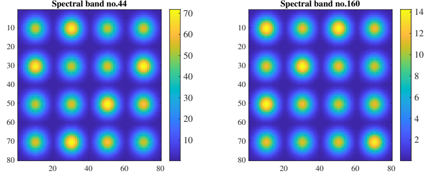
Figure 2.9: Spectral bands of the synthetic SRI with R = 7 materials.
