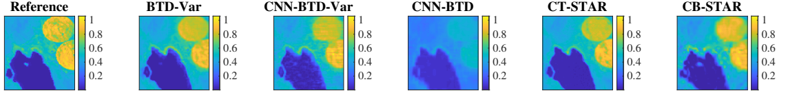
Figure 3.2: Spectral band no.40 of the SRI, Lake Tahoe.
