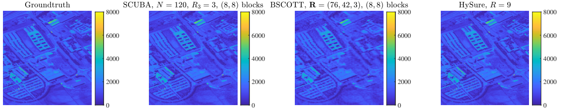
Figure 2.5: Spectral slice no.44 of the SRI, Pavia University.
