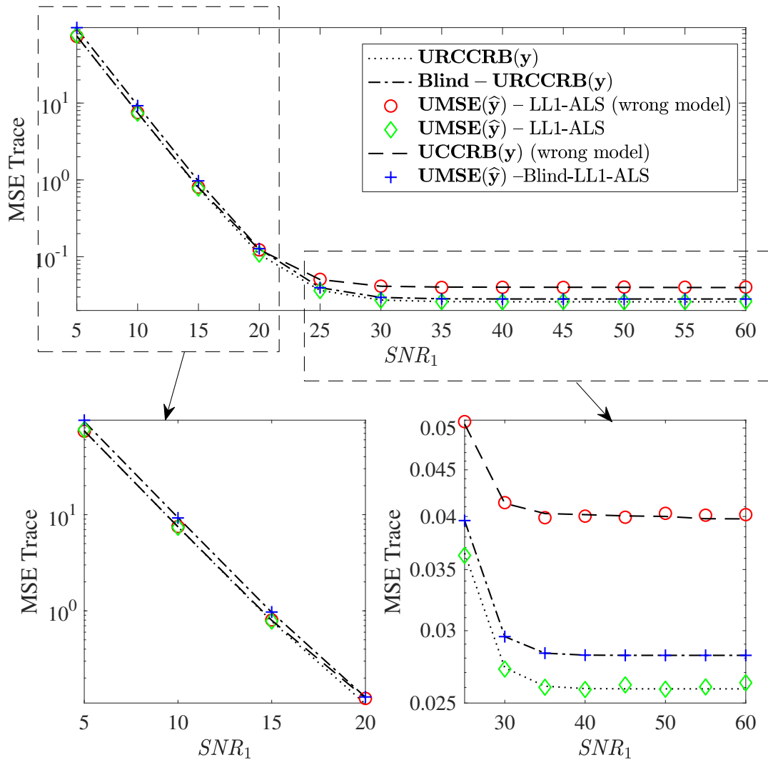
Figure 5.7: Standard UCCR B (using a false model), RCCR B , Blind-RCCR B , and UMSE for the parameter \mathbf{y} and different models; close-ups for SNR_1 \leq SNR_2 (down, left) and SNR_1 > SNR_2 (down, right).
