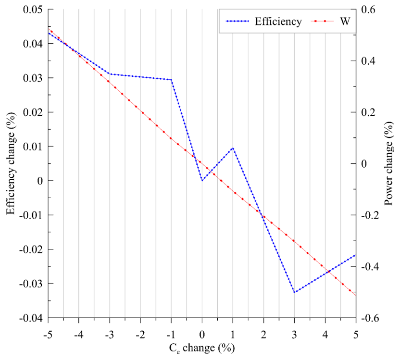
Figure 4.6: Sensitivity of the system to the C_e
