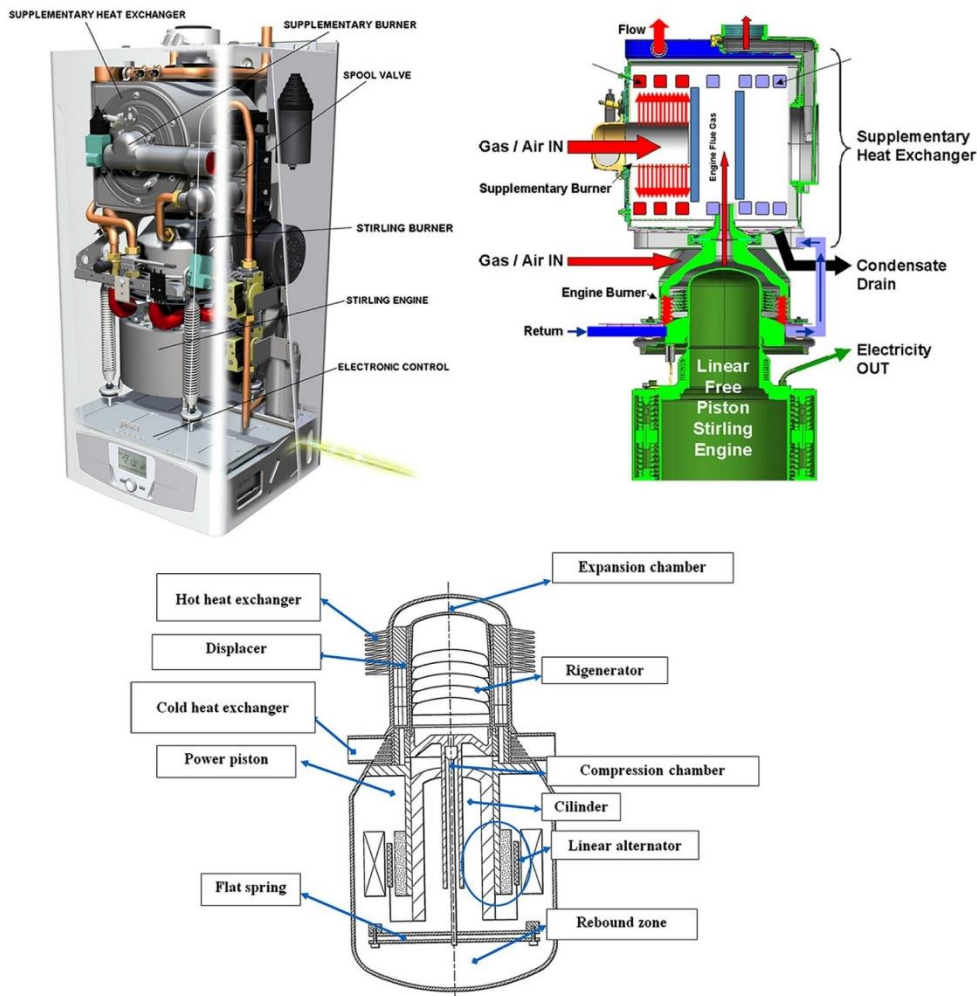
Figure 1.11: The micro-CHP Ecogen by Baxi [24]
