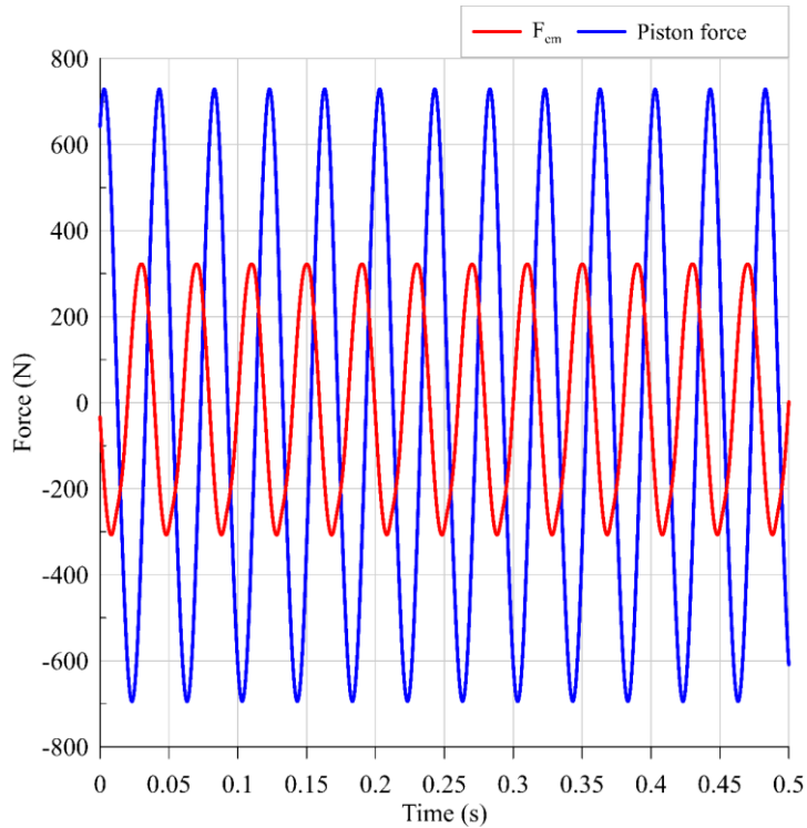
Figure 7.7: Variation of the electromagnetic and piston forces in steady state condition at reference velocity frequency of 25 Hz and amplitude of 0.55 m/s
