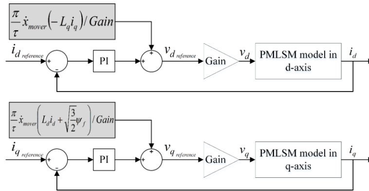
Figure 3.3: Decoupled PMLSM model for i_d and i_q
