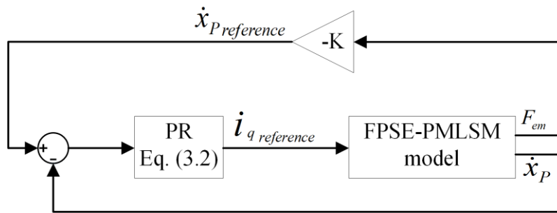
Figure 3.35: Identifying reference velocity based on electromagnetic force
