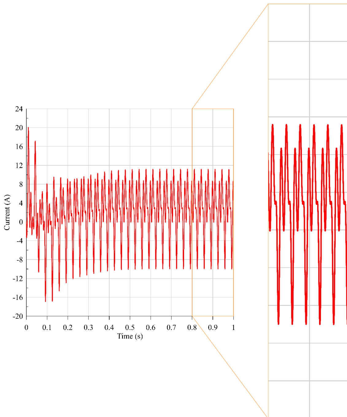
Figure 3.17: i_a current of the FPSE-PMLSM system
