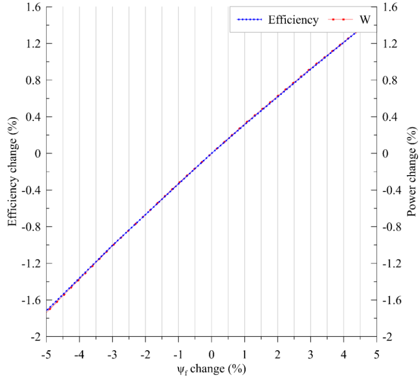
Figure 4.1: Sensitivity of the system to the \psi_f
