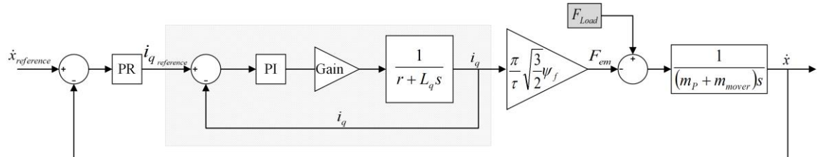
Figure 3.4: Schematic of the control system for velocity
