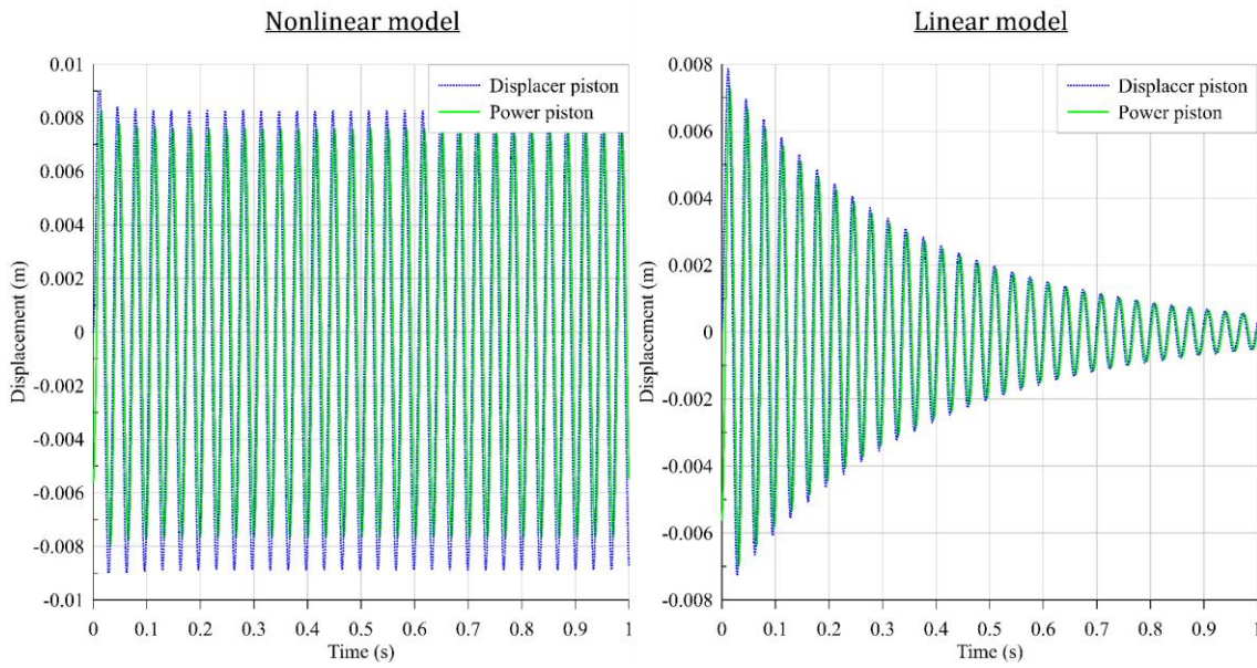
Figure 2.3: Linear and nonlinear models' results
