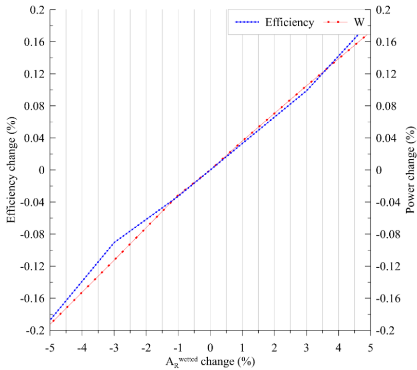
Figure 4.3: Sensitivity of the system to the A_R^{wetted}
