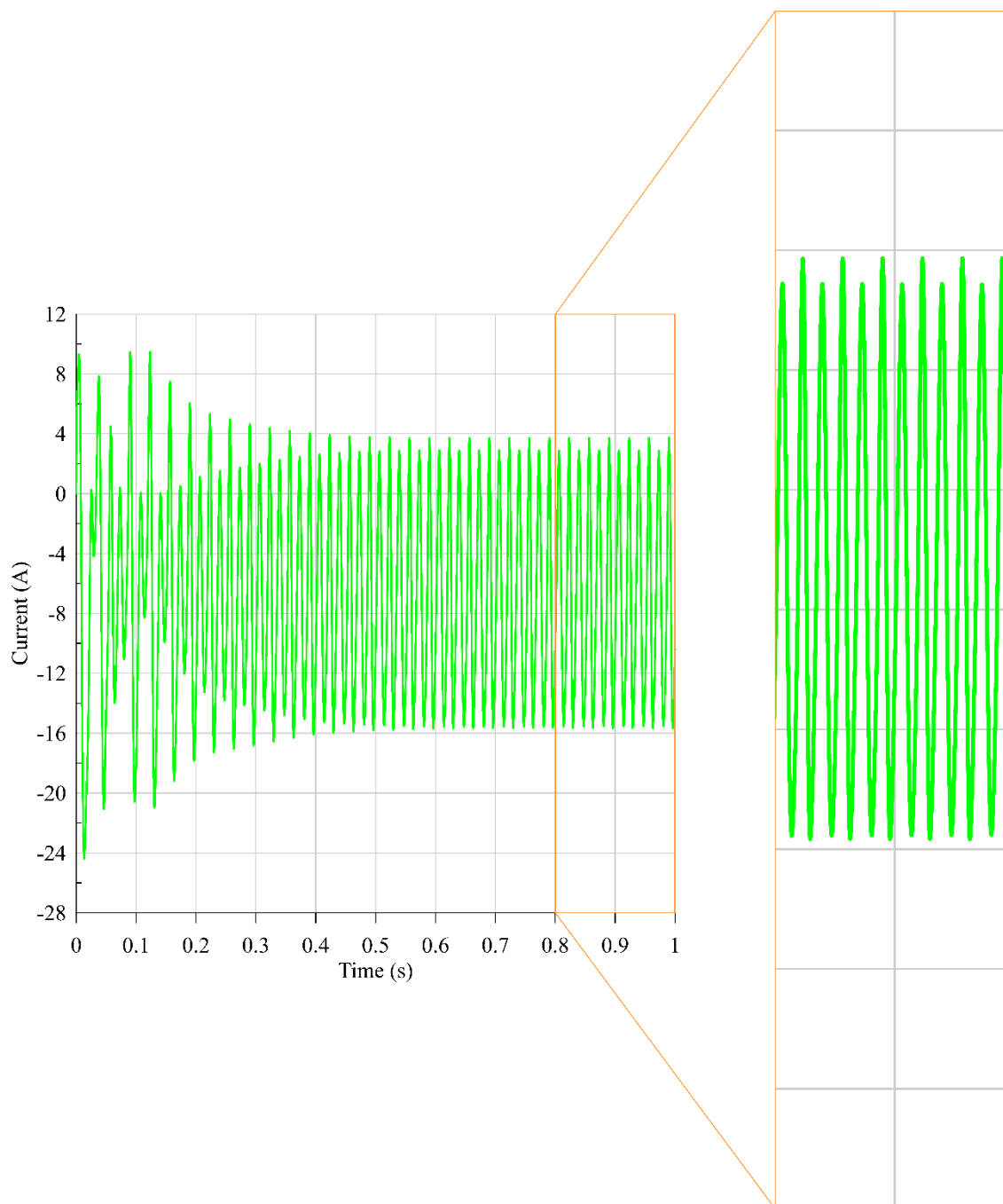
Figure 3.19: i_c current of the FPSE-PMLSM system
