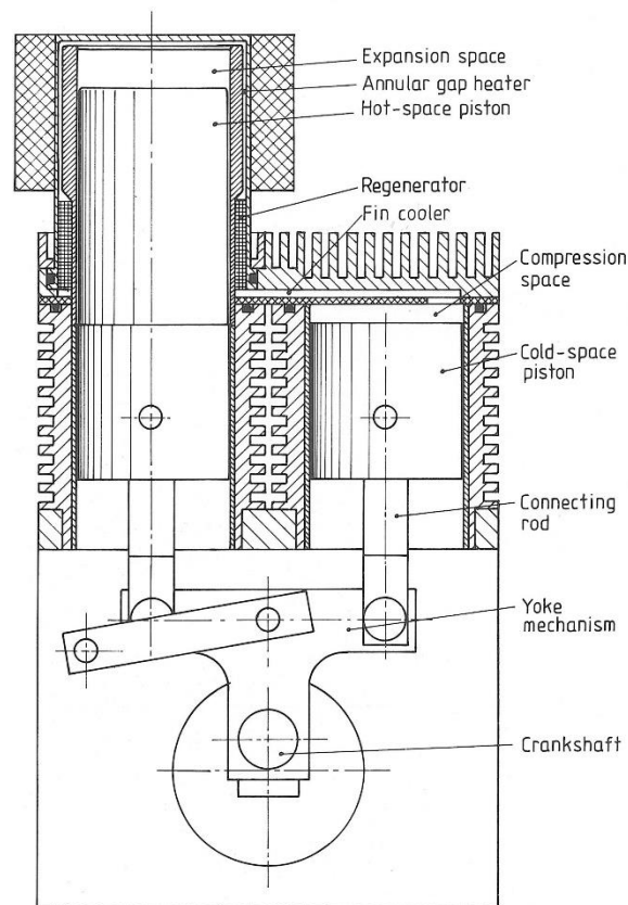
Figure 1.14: The Ross Yoke drive engine [3]
