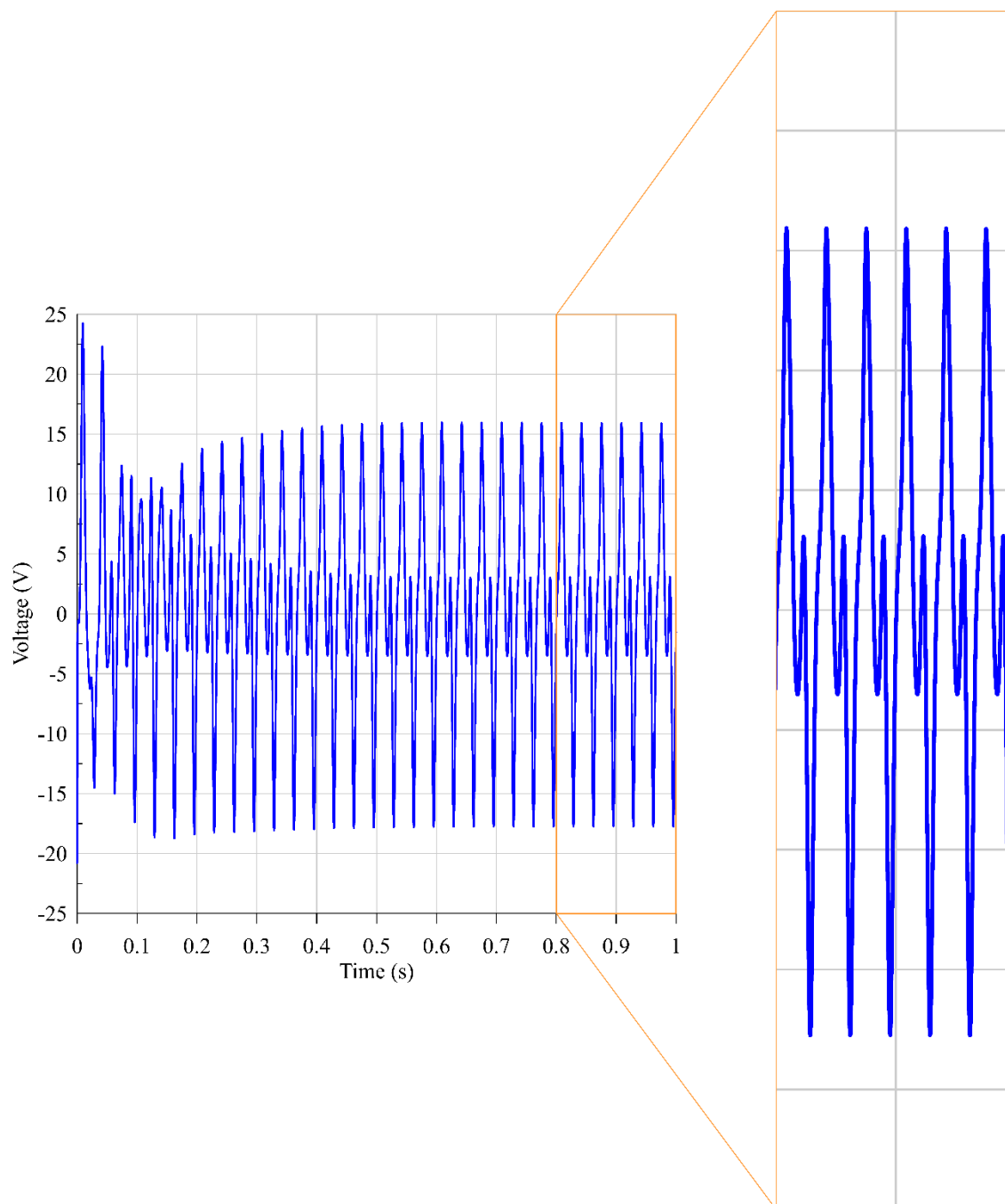
Figure 3.21: v_b voltage of the FPSE-PMLSM system
