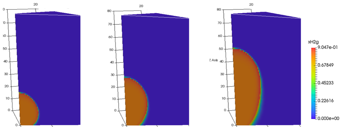
Figure III-9 Hydrogen fraction molar: after 10 days, 22 days, and 42 days of injection at the rate 0.5 kg m -2 s -1
