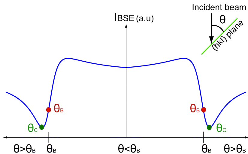
Figure III.1 – Variations of the BSE intensity with the angle between the incident beam and the diffracting plane (hkl) . The BRAGG condition corresponds to \theta = \theta_B and \theta = \theta_c is the channeling condition.
