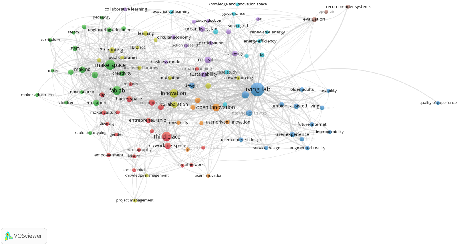
Figure 2-3: Network visualization
