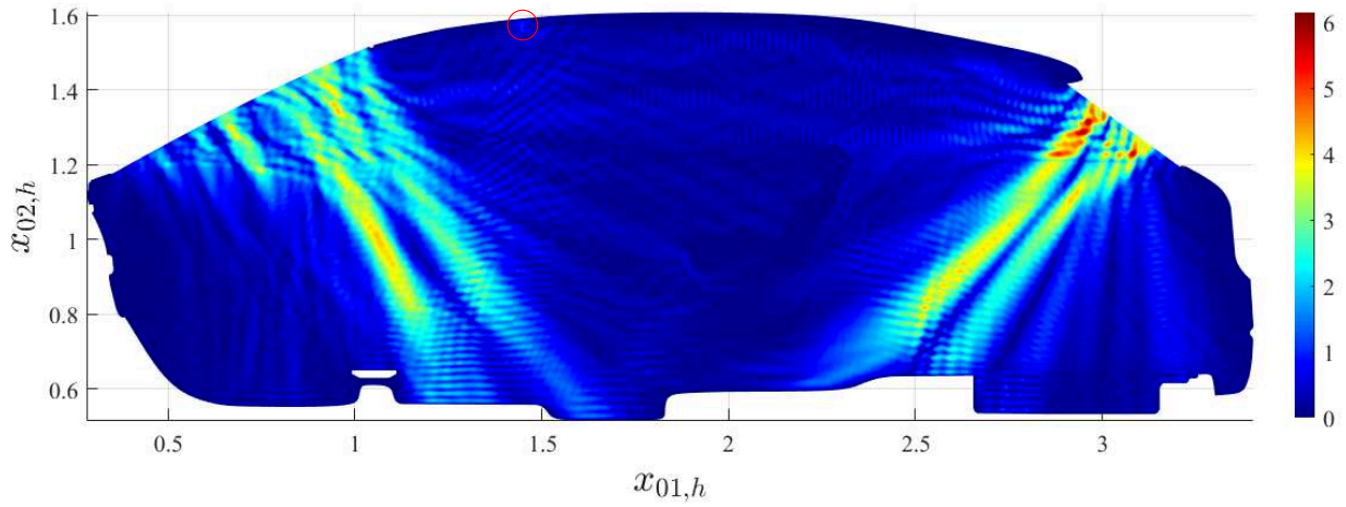
Figure 4.20: Amplitude |a_{0,h}^{(4,10)}(\mathbf{x}_{0,h})| of the field emitted from \Gamma^{s,1} for the configuration C1a.
