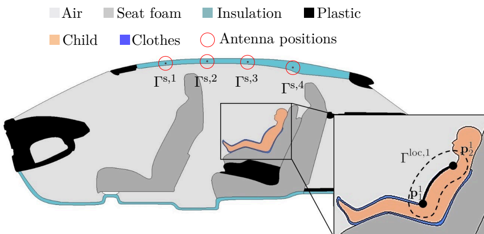
Figure 4.3: Configuration C1a.
