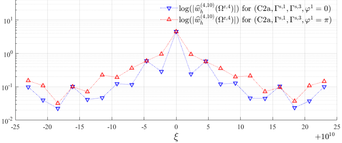
Figure 4.30: Spectrum \log(|\widehat{w}_h^{(4,10)}(\Omega^{r,4})|) emitted from both \Gamma^{s,1} and \Gamma^{s,3} in C2a, with \varphi^1 = 0 (blue) and \varphi^1 = \pi (red).
