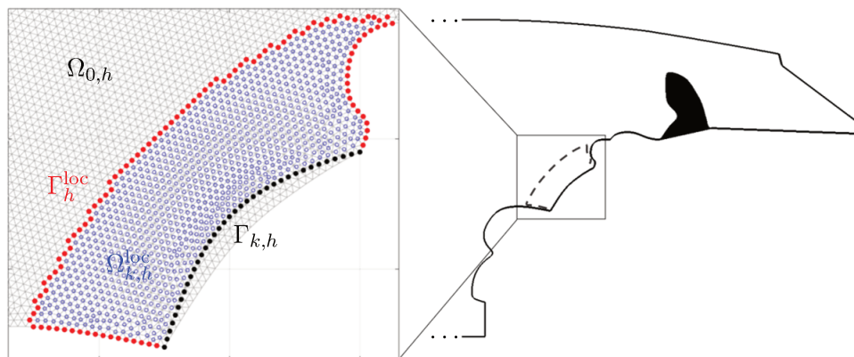
(a) Finite element triangulation and its local deformation for k = 6 .
