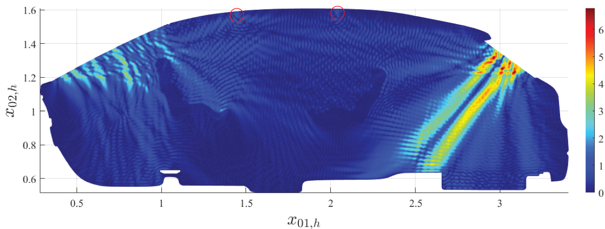
Figure 4.29: Amplitude |a_{0,h}^{(4,10)}(\mathbf{x}_{0,h})| of the field emitted from \Gamma^{s,1} and \Gamma^{s,3} for the configuration C2a.
