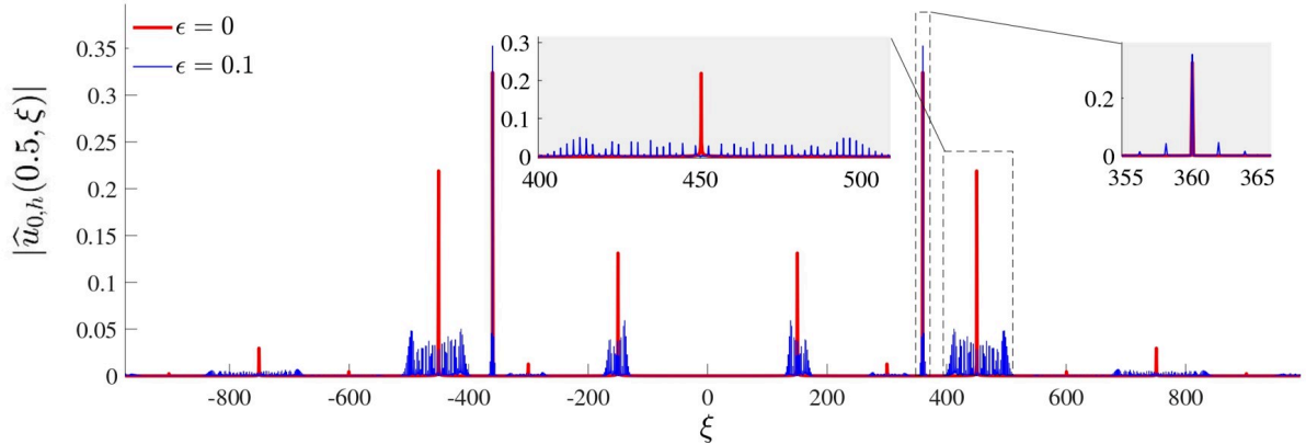
Figure 2.2: Frequency spectrum |\widehat{u}_{0,h}(0.5, \xi)| without ( \epsilon = 0 , in red) and with boundary motion ( \epsilon = 0.1 , in blue). This illustrates both the assumption on the decomposition (2.18) of v and the ansatz (2.30).
