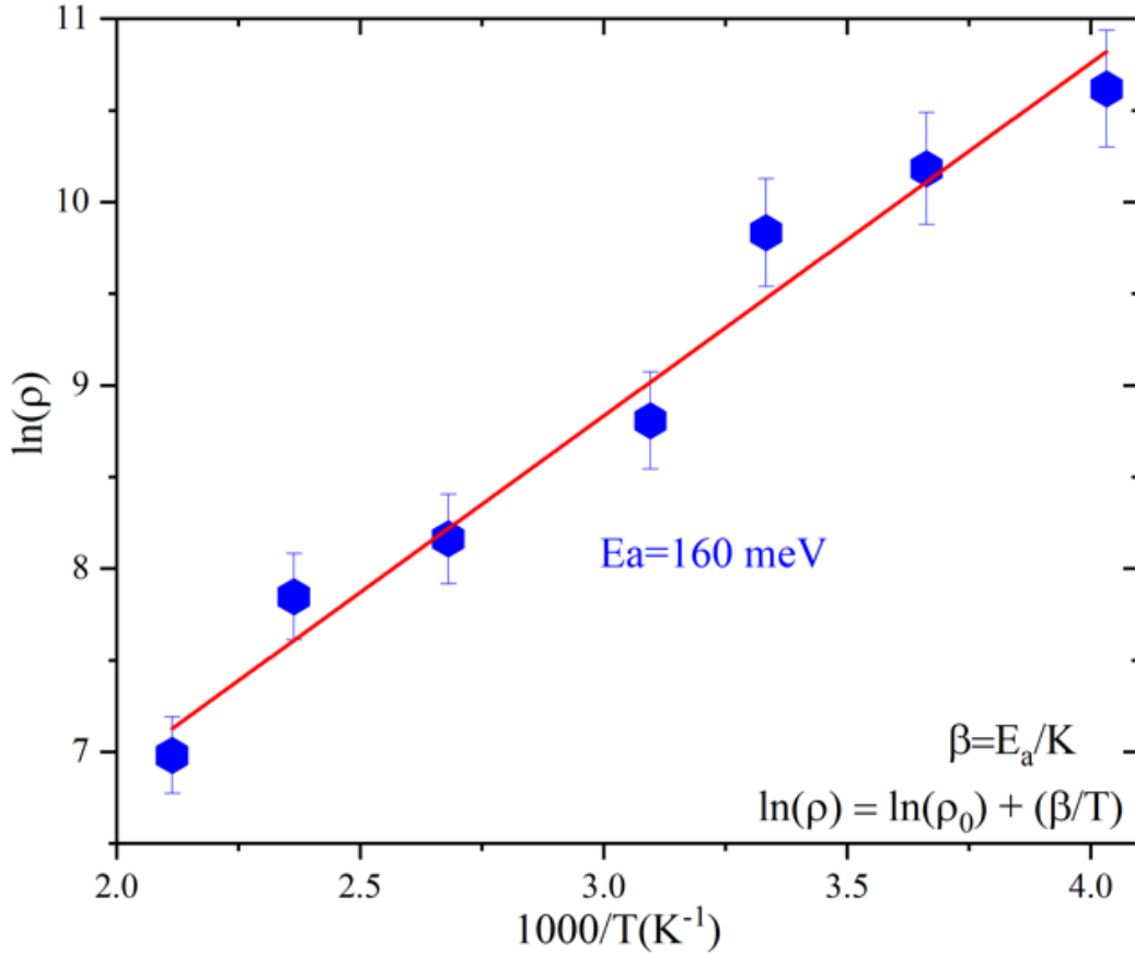
Figure 6-6: Activation energy of the 50 nm thick Mg-doped h-BN.
