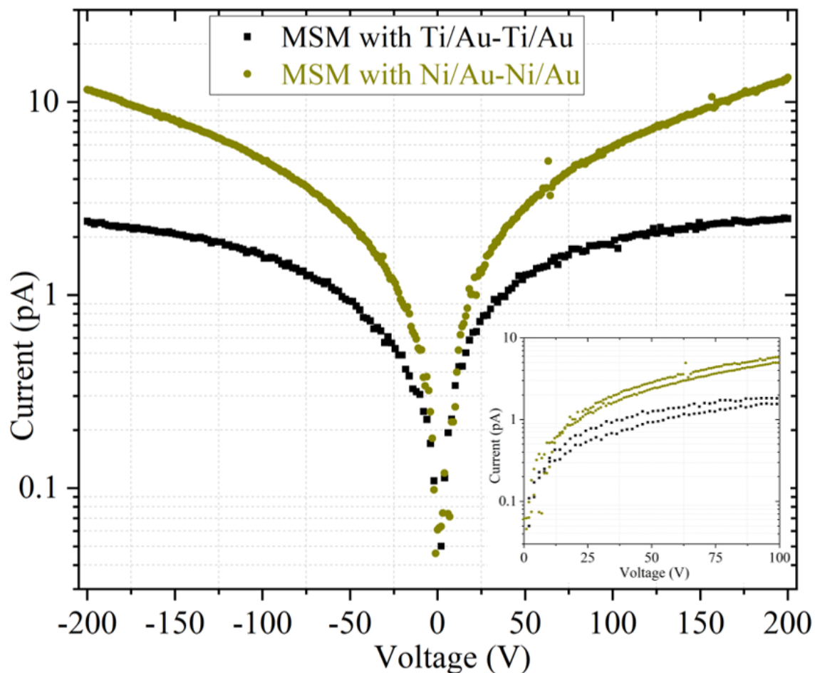
Figure 4-3: Dark current of the 2.5- \mu\text{m} thick natural h-BN MSM detectors with two different Schottky contacts (Ni/Au-Ni/Au and Ti/Au-Ti/Au). Inset shows the corresponding I- |V| curves to highlight the asymmetric behavior.
