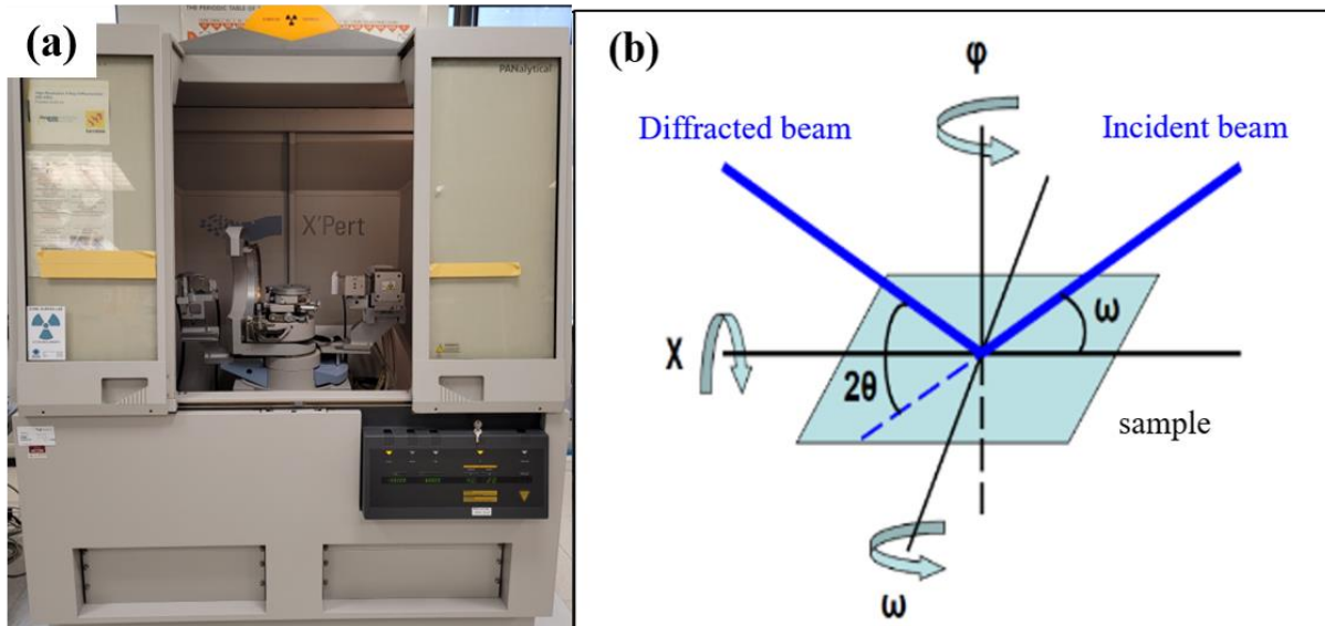
Figure 2-9: High-resolution X-ray diffraction system.
