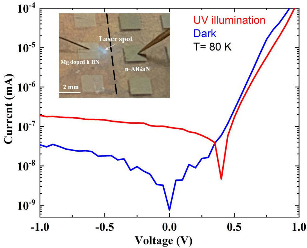
Figure 6-10: I-V curve recorded in Mg doped h-BN/n- \text{Al}_{0.58}\text{Ga}_{0.42}\text{N} (Sample F) at T = 80\text{ K} with and without UV laser illumination. The inset shows a photograph of the top view of the heterojunction with the electrical contact pad and the location of the laser spot.
