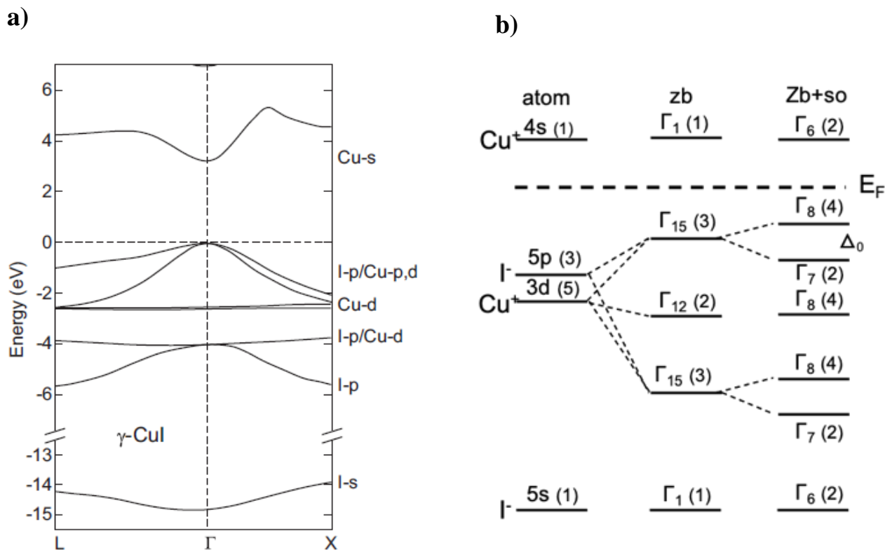
Figure 1.7: a) The electronic band structure of \gamma -CuI (calculated with GGA-PBE level) adapted from [59] b) Representation of the conduction and valence state in CuI due to s, p, and d electrons at the \Gamma -point in the cubic crystal field of the zinc blende structure “so” is referring to spin-orbit interaction. Numbers in brackets indicate the degeneracy state [60].
