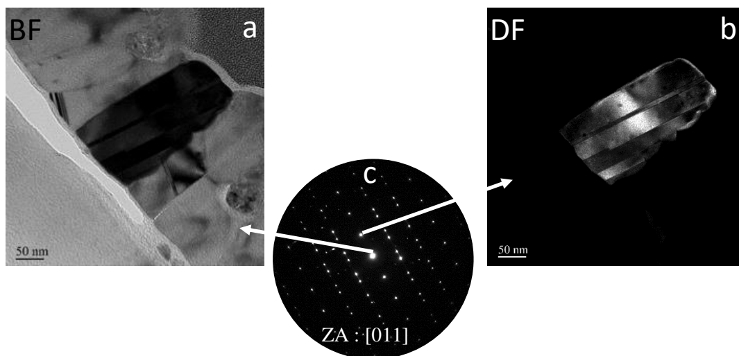
Figure 2.11: a) Bright and b) dark images as well as c) SAED pattern of a prepared \text{CuI} thin film sample synthesized with 0.15 g of \text{I}_2
