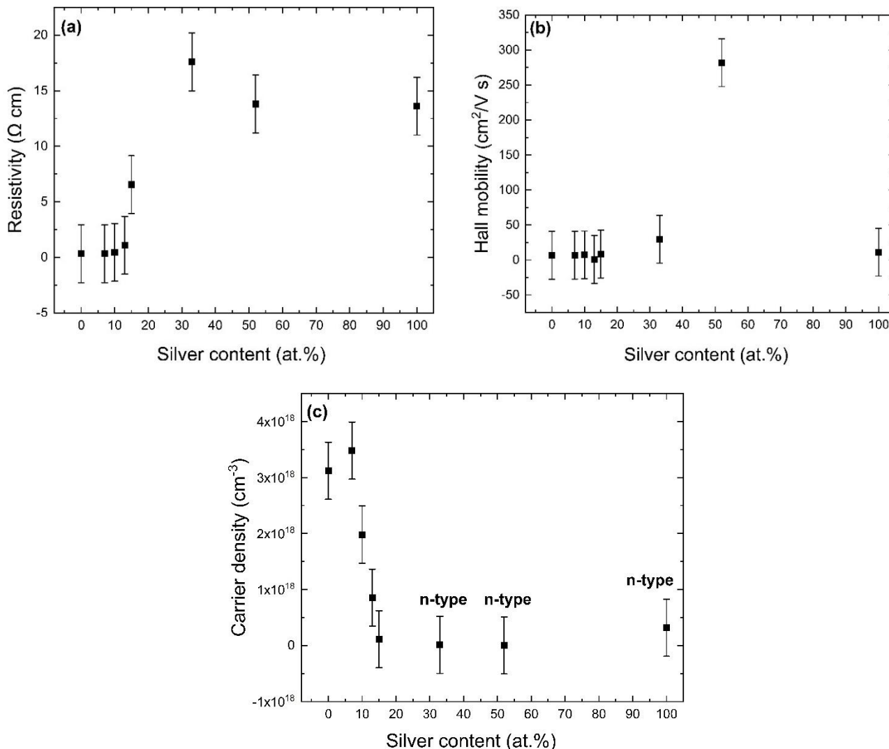
Figure 4.14: Resistivity(a), Hall mobility(b) and carrier density(c) measured for (Ag,Cu)I films depending on silver content.
