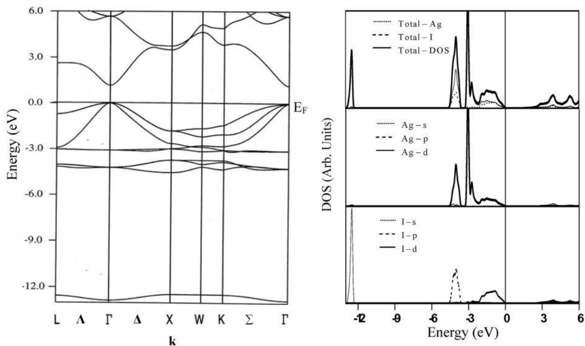
Figure 1.17: Band structure and density of states of \gamma -AgI along high symmetry directions of the first Brillouin zone adapted from [92].
