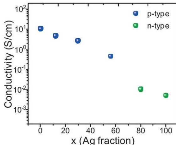
Figure 1.13 Conductivity variations for Ag_xCu_{1-x}I alloys as a function of Ag content adapted from [71].
