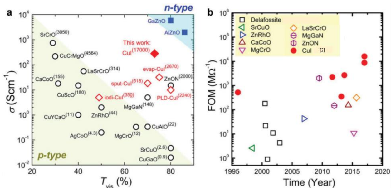
Figure 1.14: a) Electrical conductivity and averaged visible transmittances for CuI and other n- and p-type TCOs. b) Comparison of FOM over time for the reported p-type TCOs [2].
