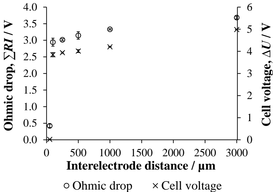
Fig. VI.10. Ohmic drop ( \Sigma RI ) of electrolyte (O) and cell voltage ( \Delta U ) (X) as a function of d_{elec} . Cathode: stainless steel, anode: BDD and j_{app} = 4 \text{ mA cm}^{-2} .
