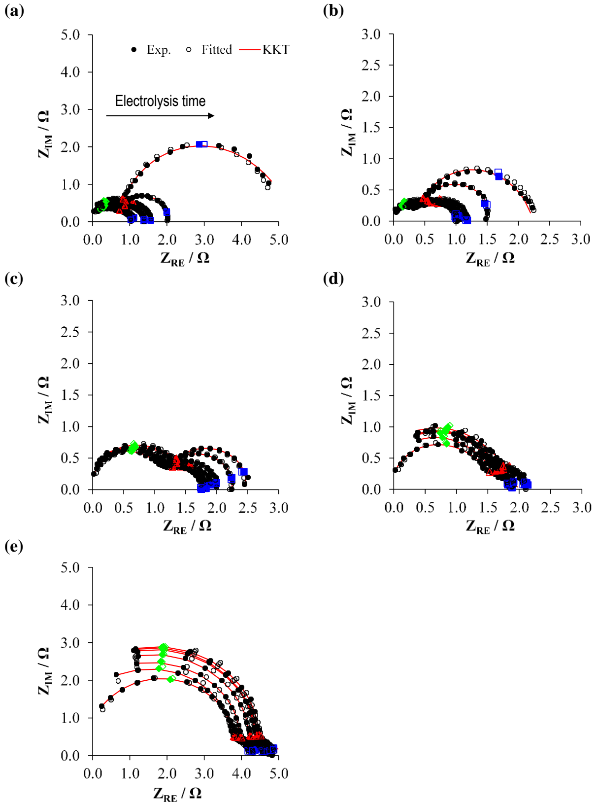
Fig. VI.12. Plots of linear KKT (—), experimental (●) and EEC theoretical (○) impedance spectra for d_{elec} of (a) 100 \mu\text{m} , (b) 250 \mu\text{m} , (c) 500 \mu\text{m} , (d) 1000 \mu\text{m} and (e) 3000 \mu\text{m} . (◆, ◇): high frequency (20 kHz), (▲, △): middle frequency (2 kHz) and (■, □): low frequency (0.2 kHz) impedance samples. Electrolysis time: 0, 0.5, 1, 2, 3, 4 and 5 h.
