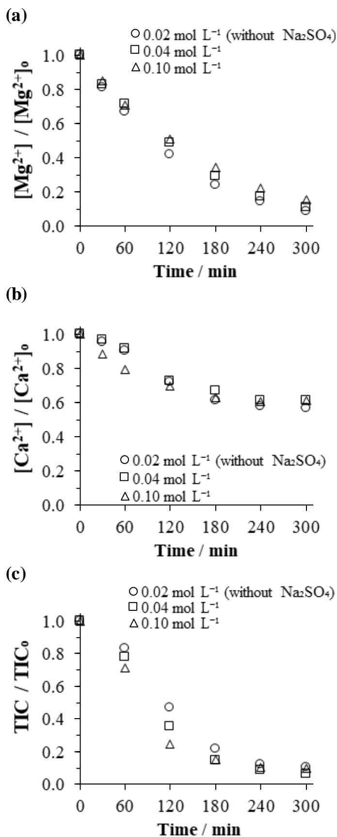
Fig. IV.4. Evolution of concentrations of (a) Mg 2+ , (b) Ca 2+ and (c) TIC during the electrolysis of artificial effluents bearing different ionic strengths of 0.02 (○) (without the addition of supporting electrolyte), 0.04 (□) and 0.10 (△) mol L -1 . Anode: BDD, cathode: stainless steel, j_{app} : 4 mA cm -2 and d_{elec} : 500 μm.
