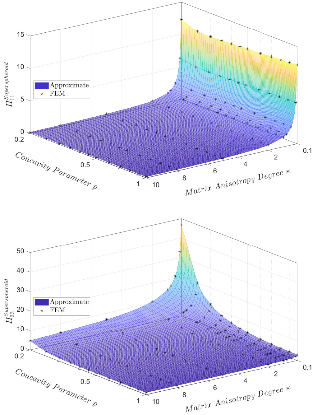
Figure 3.9: The two independent components H_{11}^{so} and H_{33}^{so} of a superspheroidal pore embedded in TI matrix, as a function of concavity parameter p and anisotropic degree of host matrix \kappa . Comparison between FEM results (star points) and approximate relations (plain surface).
