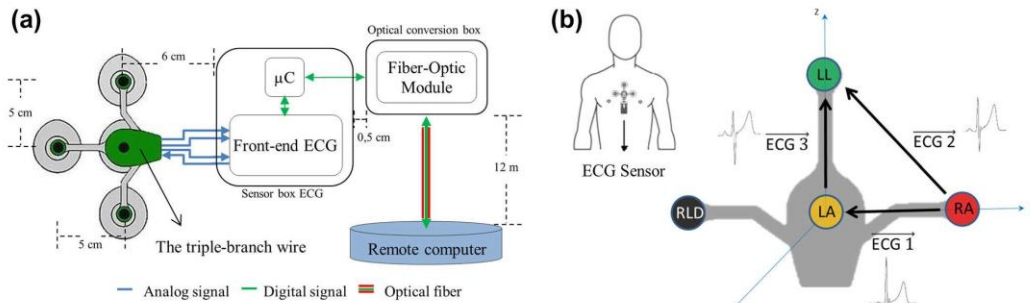
FIGURE 2. (a) Electronics design of the proposed ECG device. The copper (blue) conductor cables between the triple-branch wire and the front-end ECG system into the device are not shielded. The length of the cables is about 11 cm. The length of the optical fiber that connects the ECG sensor and the remote computer is 12 m. (b) Positioning of the RMN-compatible ECG sensor on the volunteer's chest, and measured ECG leads.
