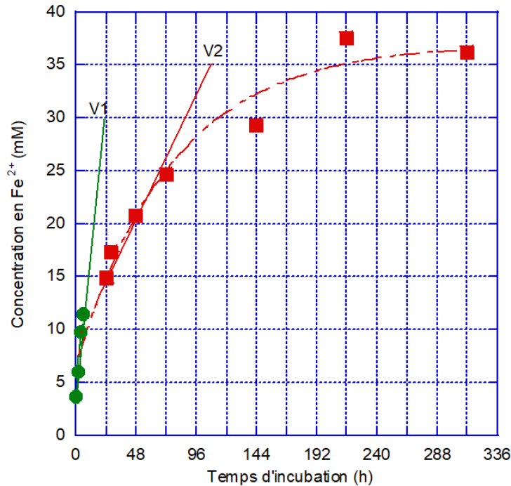
Fig 6.11: Initial rate of reduction of Fe^{3+} to Fe^{2+} based on the Fe^{2+} concentration curve produced by S. putrefaciens in FCm medium with 4 mM formiate and without NaCl: green curve corresponds to the initial rate of reduction of Fe^{3+} in the presence of only formiate (V1), while the curve in red corresponds to the initial rate of reduction of Fe^{3+} in presence of formiate and H_2 (V2).
