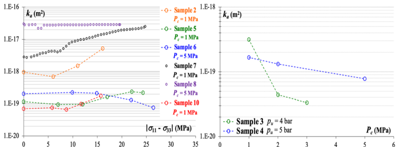
Fig. 3. 12: Left, evolution of apparent permeability k_a as a function of deviatoric stress for Samples 2, 5, 6, 7, 8 and 10. Right, evolution of apparent permeability k_a as a function of confining pressure P_c for Samples 3 and 4.
