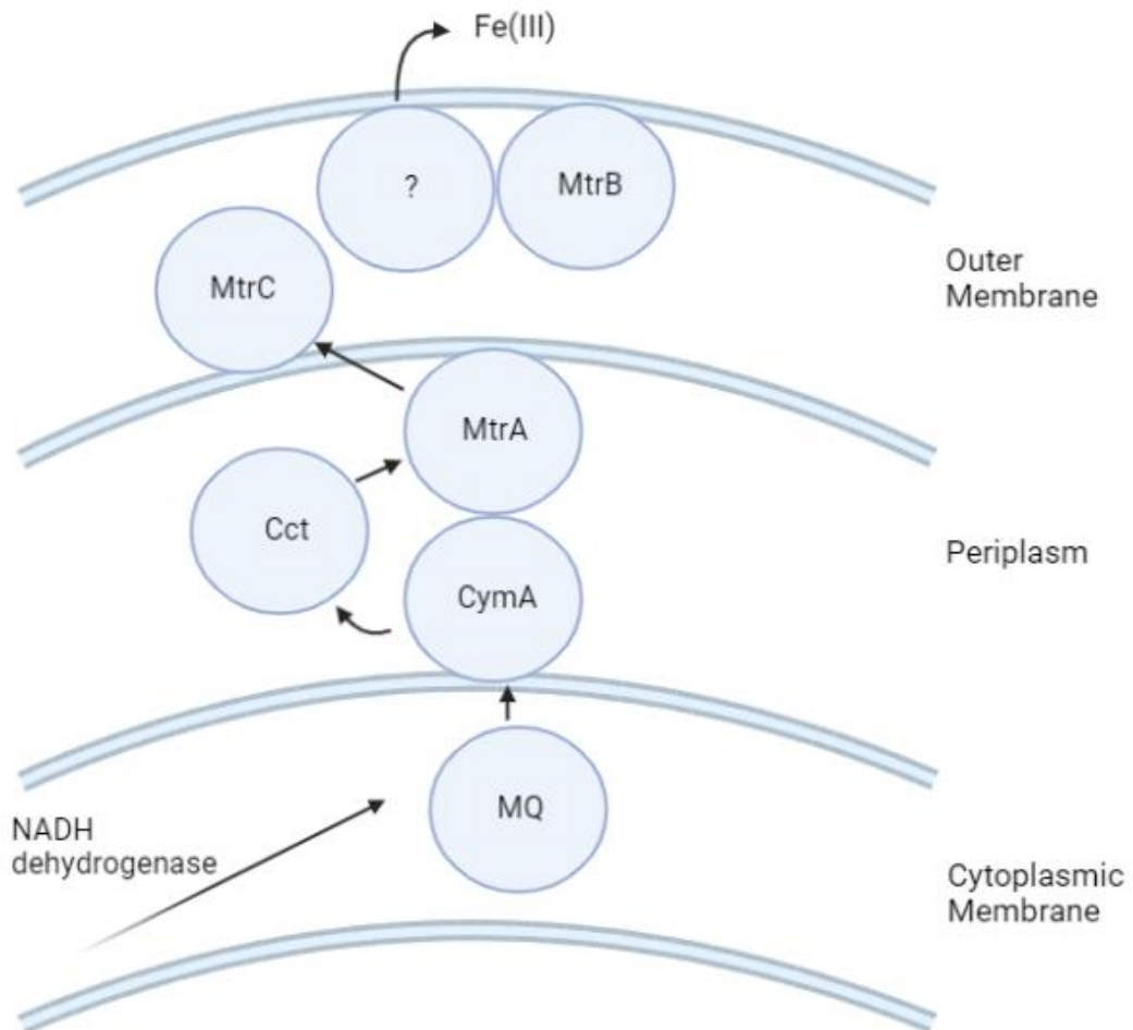
Fig 5. 6: Diagram describing to the reduction of Fe^{3+} by the S. putrefaciens membrane proteins (MtrB, MtrC and Cct involved in metal reduction, MtrA, CymA, MQ periplasmicdecahaemc-type cytochrome involved in electron transportation chain when uptaking an electron,(Beliaev et al., 2001).
