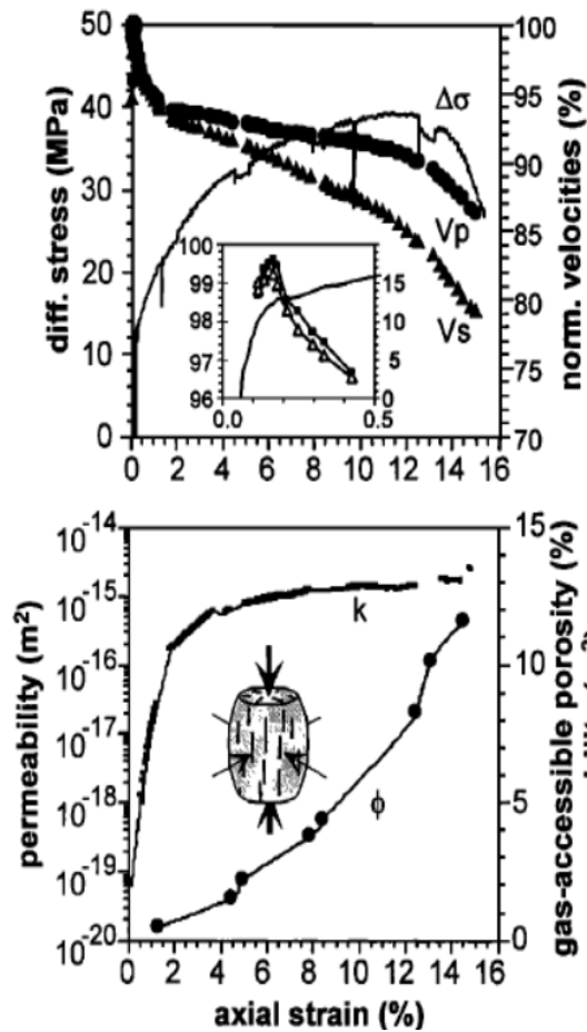
Fig 2. 20: Change of physical properties in function of strain and strength at compression controlled strain rate e=10^{-5}s^{-1} m confining pressure P_c=2MPa , temperature T=30^\circ C . Evolution of dilatancy (indicated by the decrease of V_p and V_s ) as a function of compressive strain. The crack initiation stress defining the dilatancy boundary is indicated by the reversal of V_s at \Delta\sigma=10MPa . Evolution of permeability and gas accessible porosity versus strain (Popp et al., 2001).
