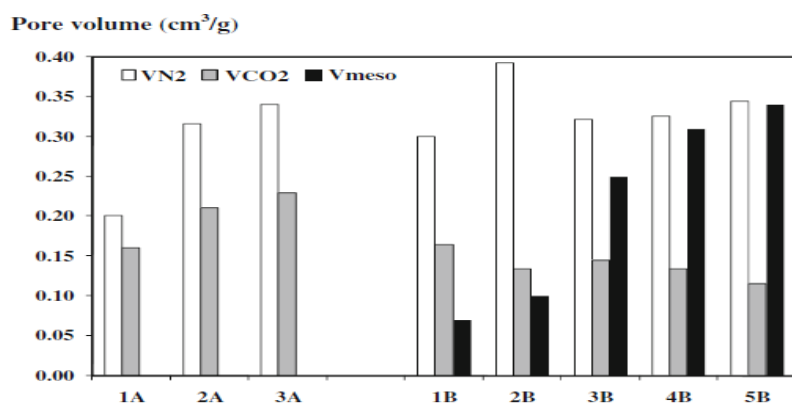
fig. 7 Pore volume of narrow micropores ( V_{CO_2} ), total micropore ( V_{N_2} ), and mesopore ( V_{meso} ),
