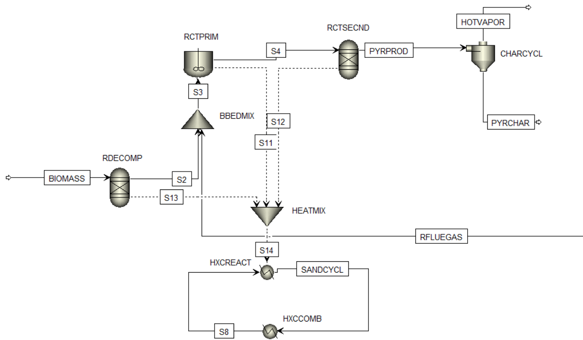
Figure 1.6. Aspen plus flowsheet of reactor model
