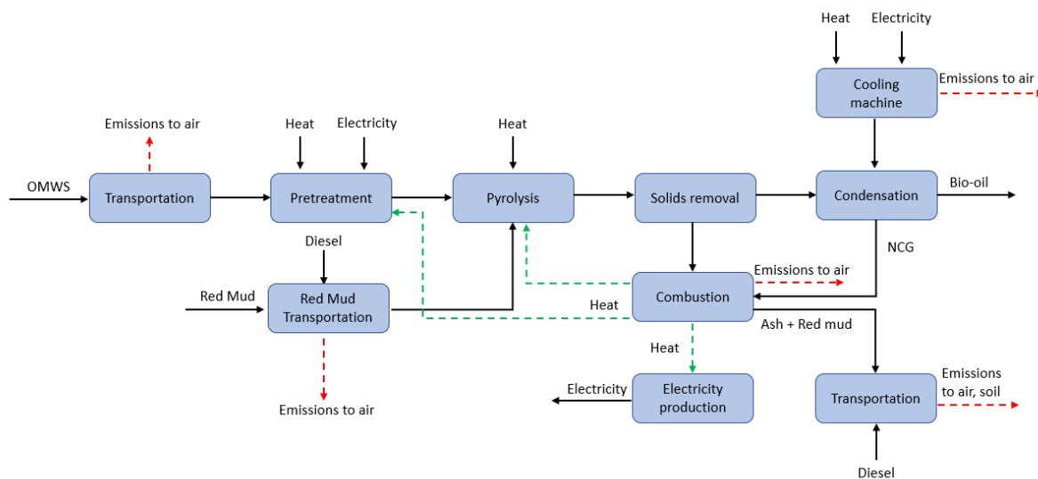
Figure 2.17. System boundaries for bio-oil production via fast pyrolysis
