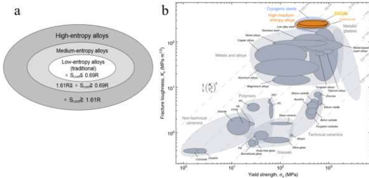
Fig. 1. 14. (a) Classification of alloys based on configuration entropy. (b) Ashby map of fracture toughness versus yield strength for various classes of materials [75].
