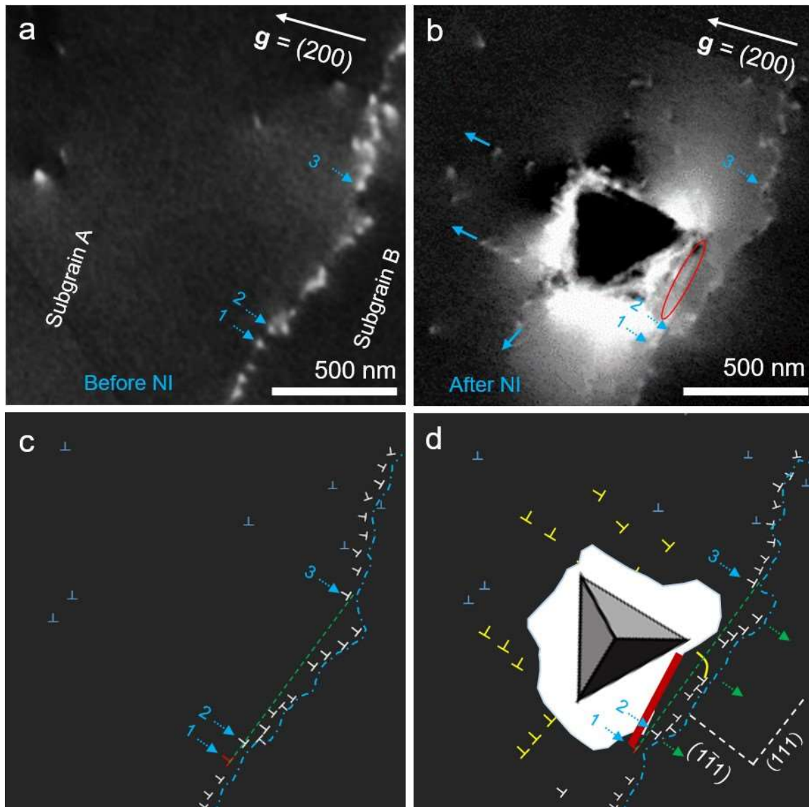
Fig. 4.9. (a) and (b) ECC micrographs before and after nanoindentation, respectively, showing the evolution of dislocation scale microstructure in the subgrain A at 0.42 μm from the LAGB (nanoindent #4 in Fig. 4.4a). (c) and (d) are schematics of (a) and (b). The blue dashed lines in (c) and (d) show the trace of the LAGB before and after deformation. The green dashed straight lines allow comparing the positions of the LAGB dislocations 1, 2, and 3 before and after nanoindentation, while the green arrows show the direction of the slight motion of LAGB dislocations. The meanings of the rest of the features are the same as in Fig. 4.6 [167].
