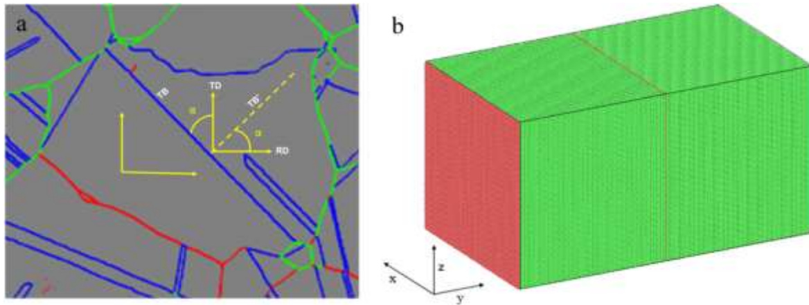
Fig. 5.11 (a) The orientation of the TB from the experiment used in the simulation. (b) Simulation box with two twin boundaries.
