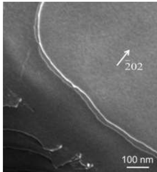
Fig. 1.16. Weak beam dark-field scanning transmission electron microscope micrograph showing Shockley partial dislocations of a dissociated dislocation in equiatomic CrCoNi MEA [90].
