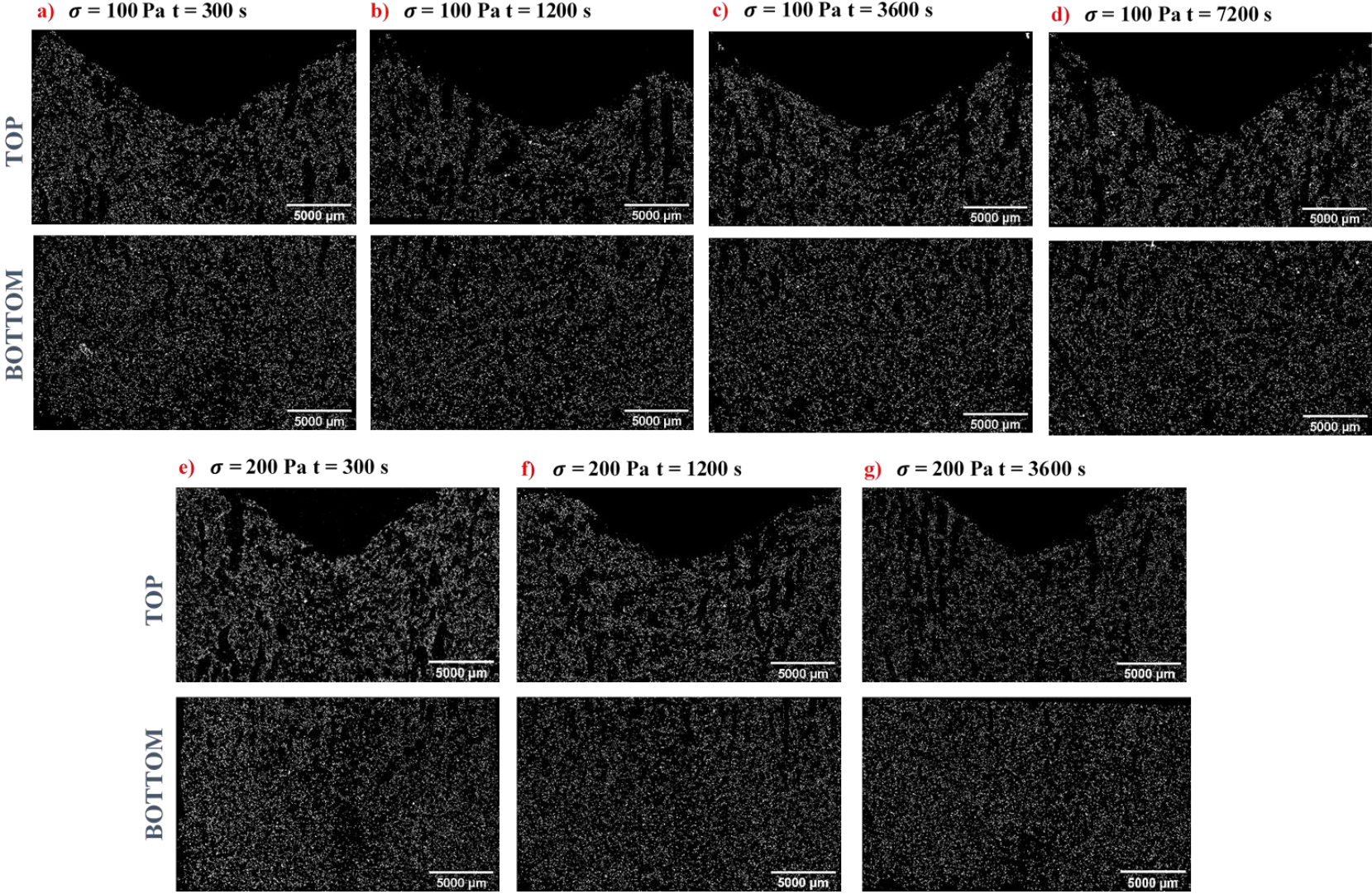
Figure V-6 - Top and bottom SEM images of the samples subject to 100 and 200 Pa stress for different durations, binarized via image treatment. Duration of the tests for the 100 Pa samples: a) 300 s, b) 1200 s, c) 3600 s, and d) 7200 s. Duration of the tests for the 200 Pa samples: e) 300 s, f) 1200 s, and g) 3600 s.
