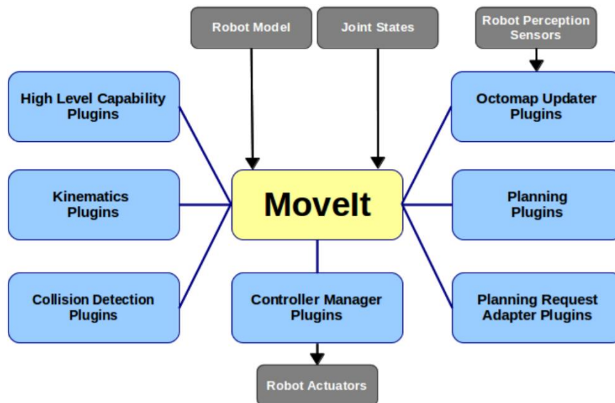
Figure 3.11 MoveIt plugin-centric framework (Coleman et al., 2014)
