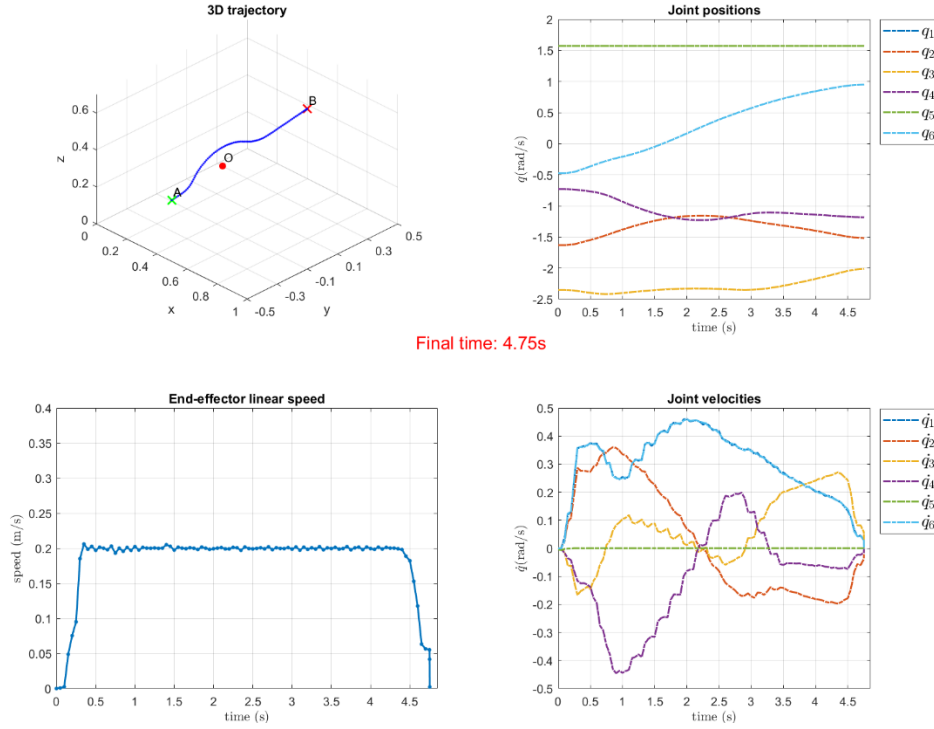
Figure 4.20 PCHIP-speed trajectory with v_{in} = 0.200\text{m/s} for case (d): 3D position trajectory, joint positions, joint velocities, and estimated end-effector linear speed
