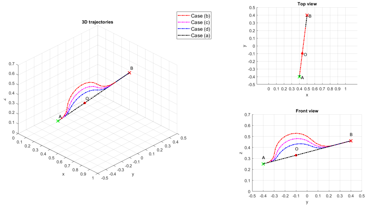
Figure 3.16 Resulting end-effector positions in the Cartesian space
