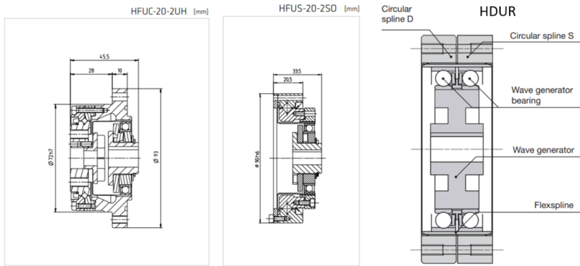
Figure 2.6 Harmonic Drive schematics for HFUC, HGUS and HDUR types
