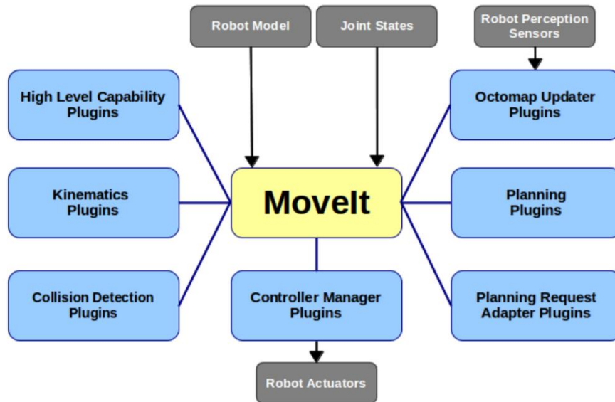
Figure 3.11 MoveIt plugin-centric framework (Coleman et al., 2014)
