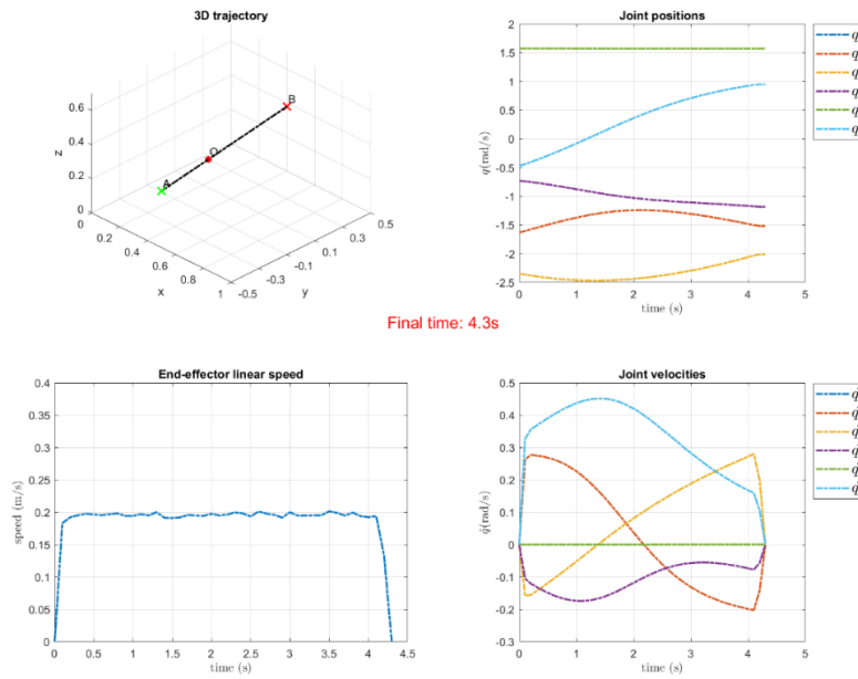
Figure 4.17 PCHIP-speed trajectory with v_{in} = 0.200\text{m/s} for case (a): 3D position trajectory, joint positions, joint velocities, and estimated end-effector linear speed
