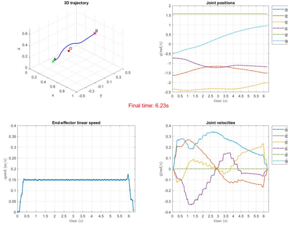
Figure 4.16 PCHIP-speed trajectory with v_{in} = 0.149\text{m/s} for case (d): 3D position trajectory, joint positions, joint velocities, and estimated end-effector linear speed
