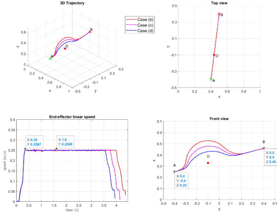
Figure 4.25 PCHIP-speed obstacle avoidance trajectories with v_{in} = 0.250\text{m/s}
