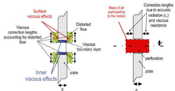
Figure 5.7: Physical phenomena involved in one perforation [18].
