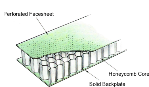
Figure 5.6: Typical single degree of freedom perforated panel
