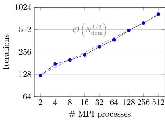
Figure 5.14: Number of GMRES iterations to reach a relative residual of 10^{-6} for the 1 BPF problem.
