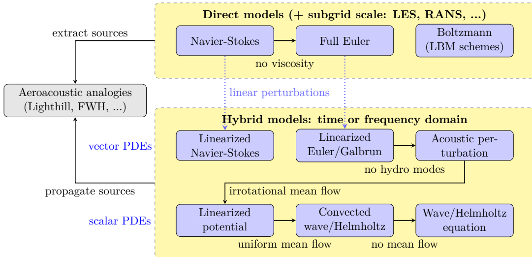
Figure 5: Overview of some common computational aeroacoustics models. Adapted from [36].
