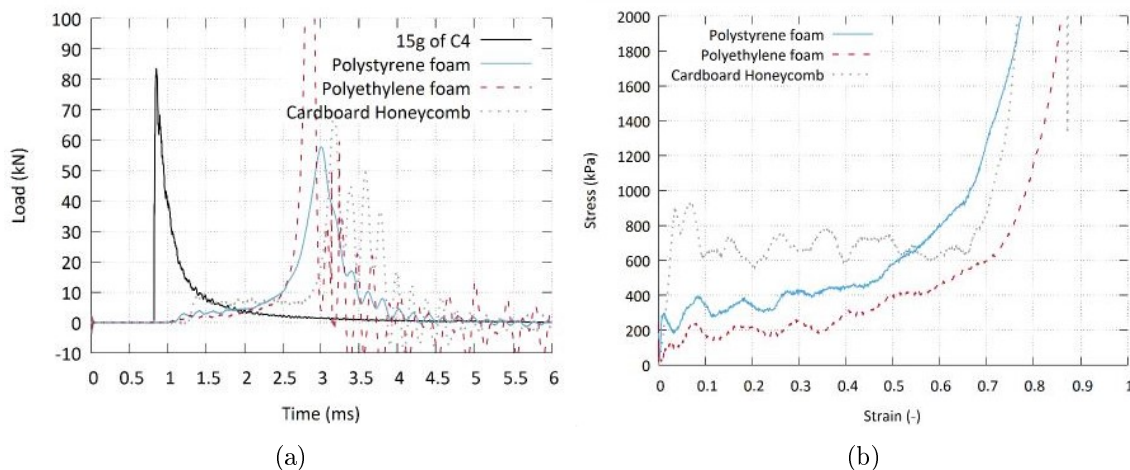
Figure 1.7: (a) Transmitted load to the target with and without cellular material (b) stress-strain curves of the tested structures under blast compression [32].
