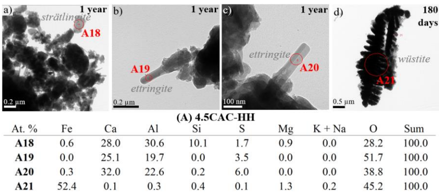
Figure 3.29 TEM images and the atomic composition of crystalline phases in the (A) 4.5CAC-HH paste sample
