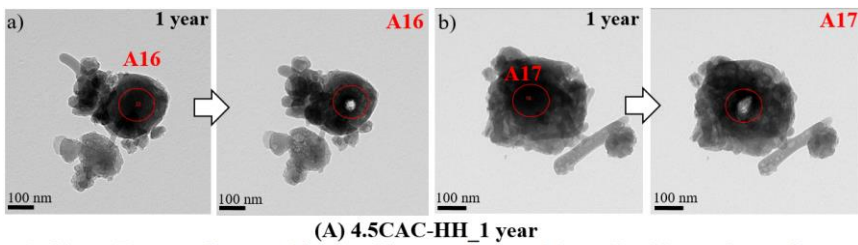
Figure 3.27 TEM images, diffraction patterns and the atomic composition of Fe-containing gels in the (A) 4.5CAC-HH paste sample
