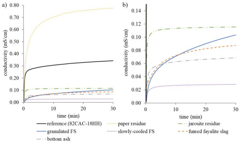
Figure 2.23 Conductivity measurements on raw materials using 0.5 g/L suspension in deionized water at 20°C
