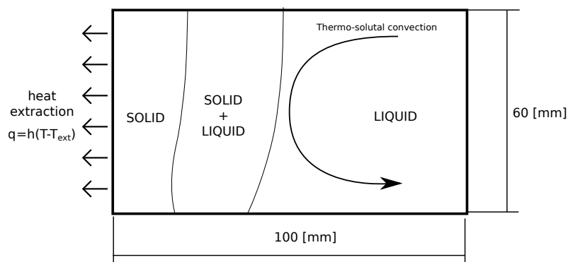
Figure 5.3 – Schematic of the 2D solidification domain in the Hebditch-Hunt case (Sn - 5 wt.% Pb alloy) with the chill heat transfer parameters: h=300 \text{ Wm}^{-2}\text{K}^{-1} and T_{\text{ext}}=25 \text{ }^\circ\text{C}
