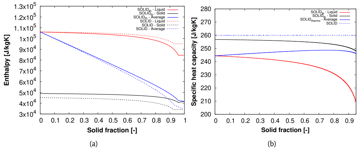
Figure 5.8 – Evolution of a) phase and average enthalpy and b) specific heat capacity obtained from SOLID th and SOLID thermo during Scheil solidification
