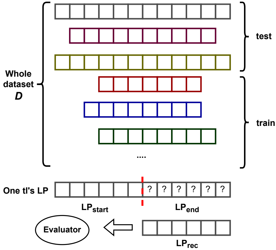
Figure 4.1: Evaluation procedure for one LP_{rec} .
