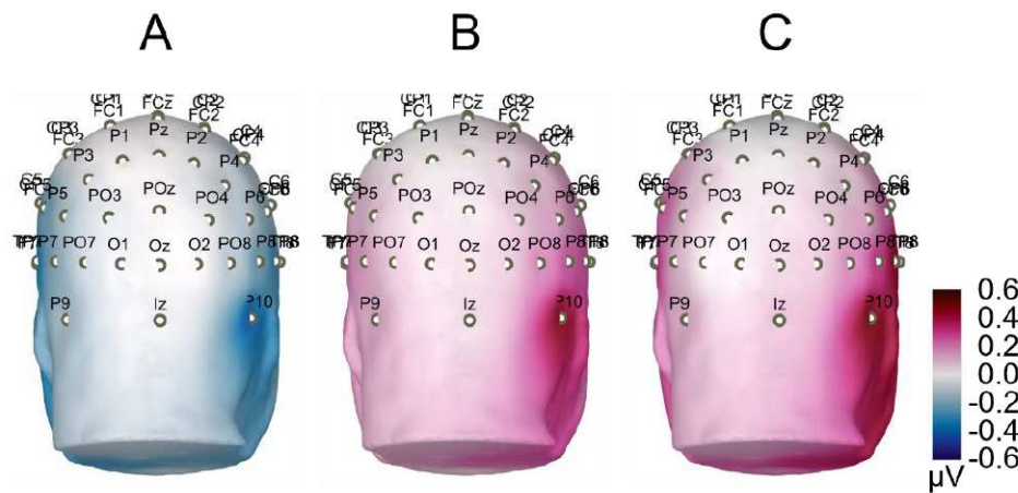
Figure 79: Topographical map of amplitude subtraction between phases at the oddball frequency (1.176 Hz). Only significant differences are shown. A : amplitude difference between before and during tDCS when Iddis with upright faces was presented. B and C : amplitude difference between during and after tDCS when Iddis with upright ( B ) and inverted ( C ) faces were presented.
