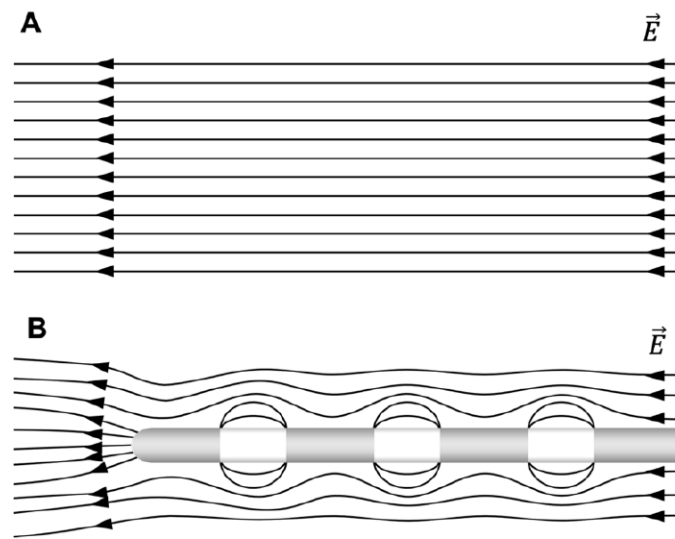
Figure 85: Schematic representation of a uniform electric field without (A) and with an SEEG electrode within (B). Electric field lines are bent as a function of the material conductivity: inward when the conductivity is higher (conductive parts in gray), outward when the conductivity is lower (insulating part in white).
