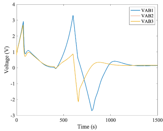
Figure 4-113 V AB voltage of each series converter.
