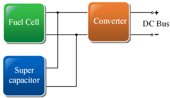
Figure 2-19 Fuel cell directly connected with supercapacitor.
