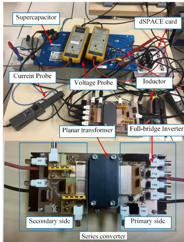
Figure 2-49 Test bench.
