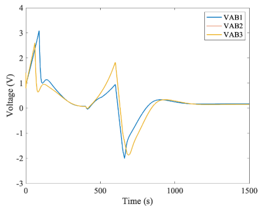
Figure 4-107 Voltage V_{AB} of each series converter.
