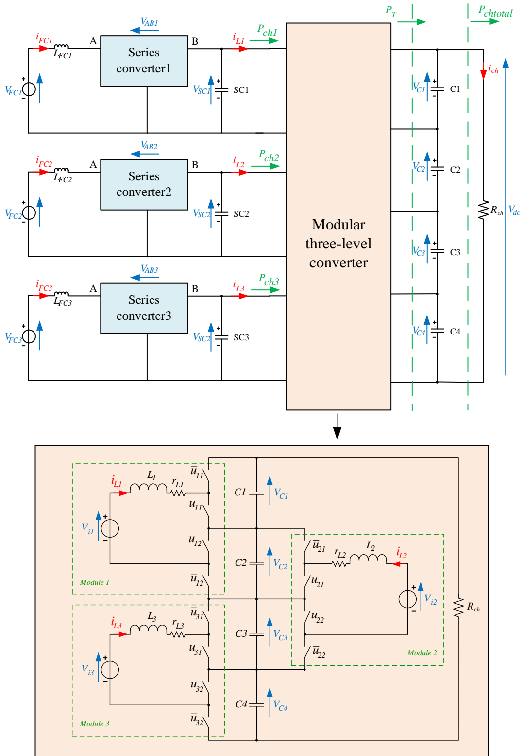
Figure 4-92 Proposed architecture.
