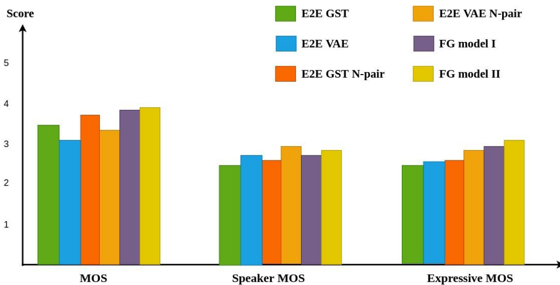
Figure 6.6 – Bar plots for results obtained from subjective listening tests on autoregressive TTS systems
