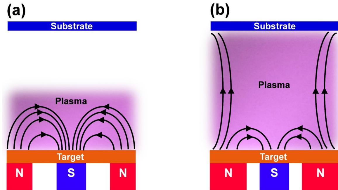
Figure 2.2. Schematic of the magnetic configuration and plasma confinement in balanced (a) and unbalanced (b) magnetrons.
