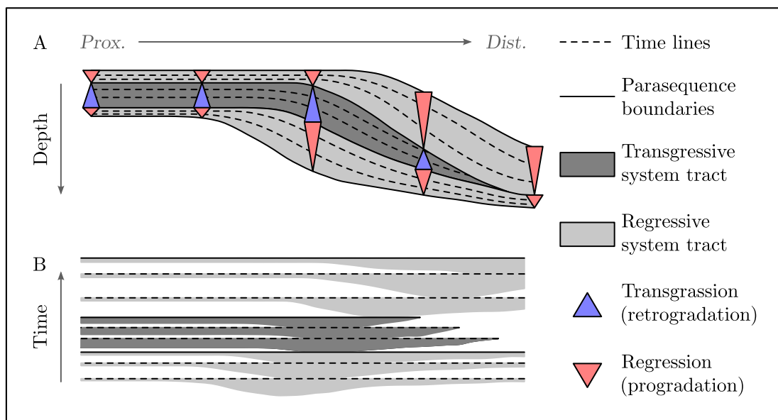
Figure 1.5: Successive transgressive and regressive parasequences corresponding to intervals observed at different scale of depth and time (Posamentier and Vail, 1988b; van Wagoner et al., 1990). Inspired by Kedzierski et al. (2008). (A) Depth cross-section and (B) time cross-section (Wheeler diagram; Wheeler (1958)). Re-draw from Baviile et al. (2022).
