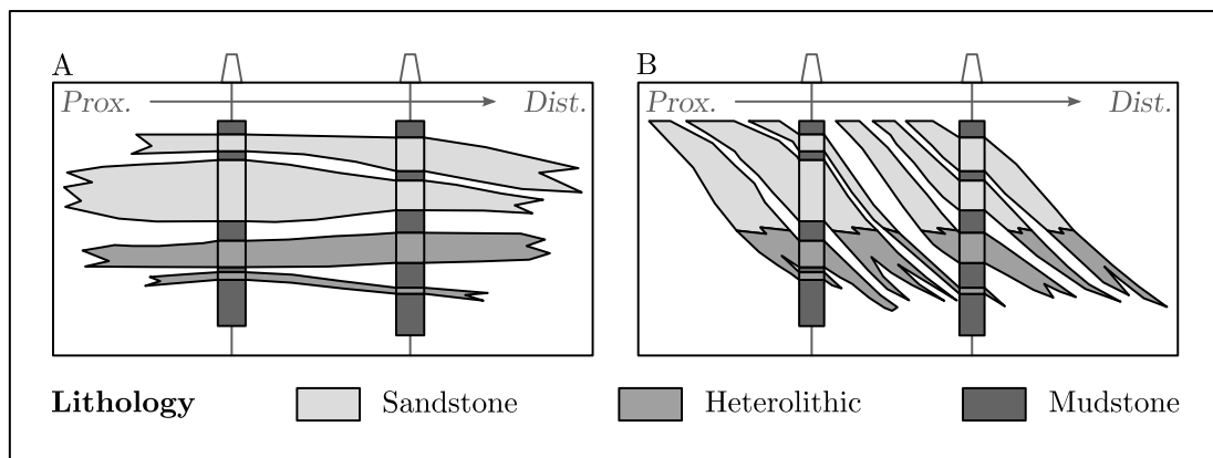
Figure 1.13: An example of lithology interpretation along two wells and their (A) lithostratigraphic and (B) chronostratigraphic geological layer interpolation and extrapolation from the same data set. Modified from Ainsworth et al. (1999) ; Baville et al. (2022) .
