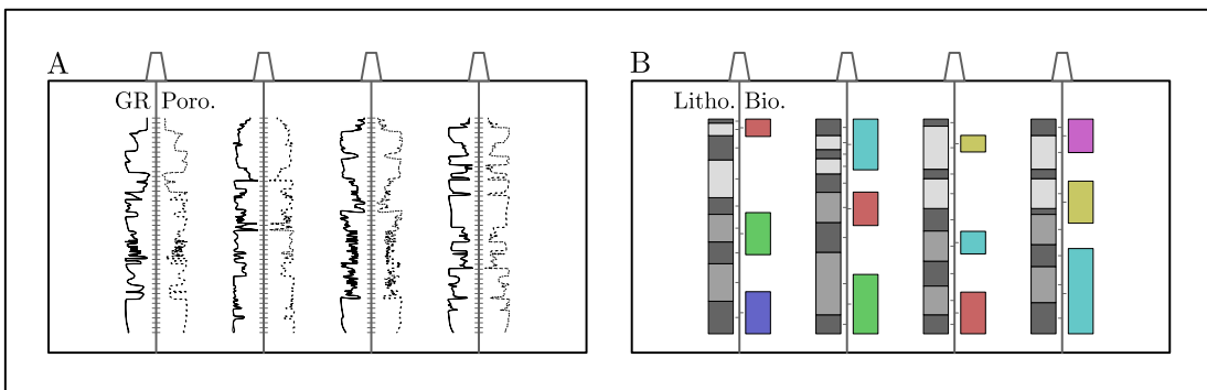
Figure 1.14: Illustration of the two types of well data and their associated well markers: (A) well logs (gamma ray and porosity) and regularly sampled well markers and (B) well regions (lithology and biozones) and irregularly sampled well markers.
