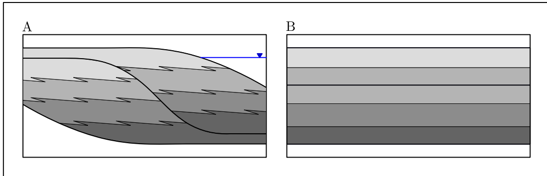
Figure 1.10: Geometry of clinoforms along a shoreline with redistribution by wave action or tidal currents (laterally to the river mouth). (A) Dip direction cross-section. (B) Strike direction cross-section. Modified from Baville et al. (2022) .
