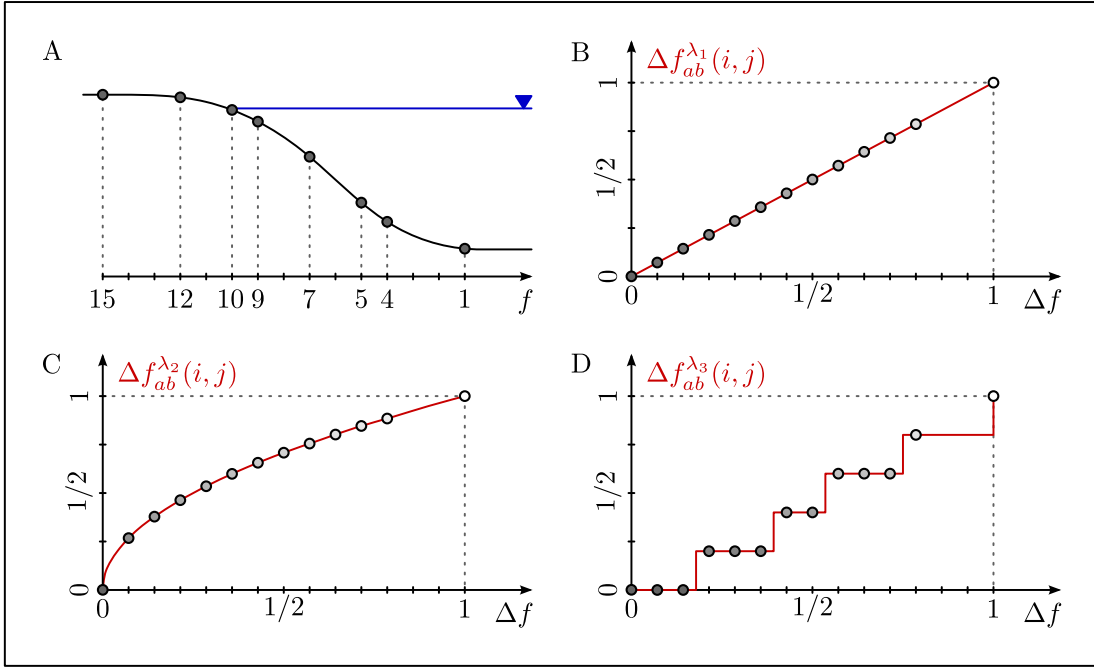
Figure 3.3: (A) Sedimentary facies f interpreted along a typical paleogeographic depositional profile and encoded from the most deep ( f = 1 ) to the most shallow ( f = 15 ). (B-C-D) \Delta f_{ab}^{\lambda}(i, j) is the relative facies variation \Delta f_{ab}(i, j) composed by the discretization function \lambda which characterizes possible relationship between several values of facies variations (Equation (3.4)).
