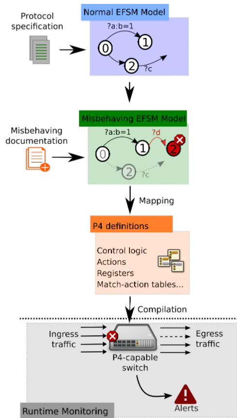
Figure 3.3: Approach overview
