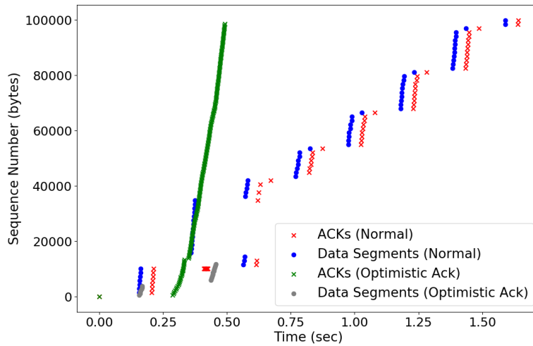
(b) Reaction
