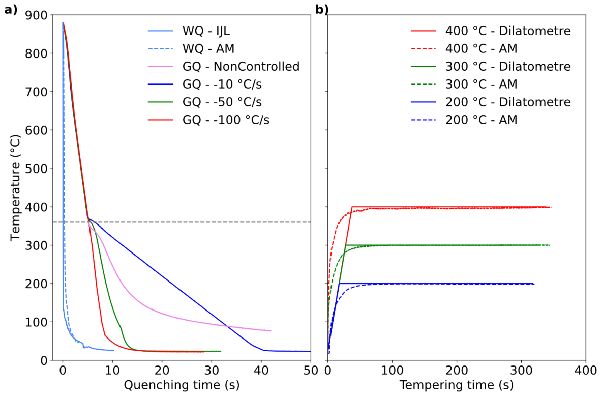
Figure 7 : a) Cooling paths applied to the 0.2C steel, WQ (in light blue) refers to water quench while GQ to gas quench with controlled temperature schedules (-10 °C/s in blue, -50 °C/s in green and -100 °C/s in red) and without temperature control (natural cooling in light violet). b) Tempering treatments applied in the present study, the continuous line refers to dilatometer trials while the dashed ones to the bath heat treatments applied at AM. Red lines refer to 400 °C tempering, while green ones to 300 °C and blue ones to 200 °C respectively.
