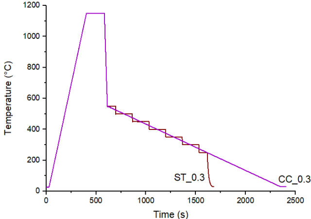
Figure. IV. 18: Heat treatments for ST_0.3 and CC_0.3 experiments.
