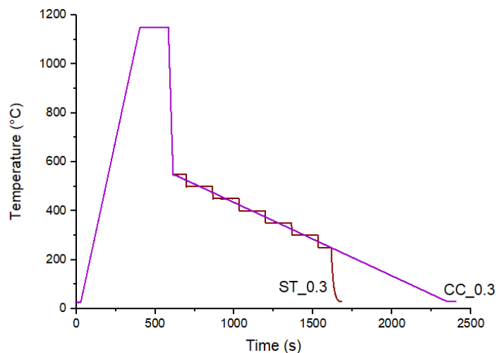
Figure. III. 23: Studied heat treatment representative of a forging condition with a constant cooling rate at 0.3^{\circ}\text{C/s} below 550^{\circ}\text{C} (purple) and multistep experiment ST_0.3 (dark red) with a mean cooling rate at 0.3^{\circ}\text{C/s} below 550^{\circ}\text{C} .
