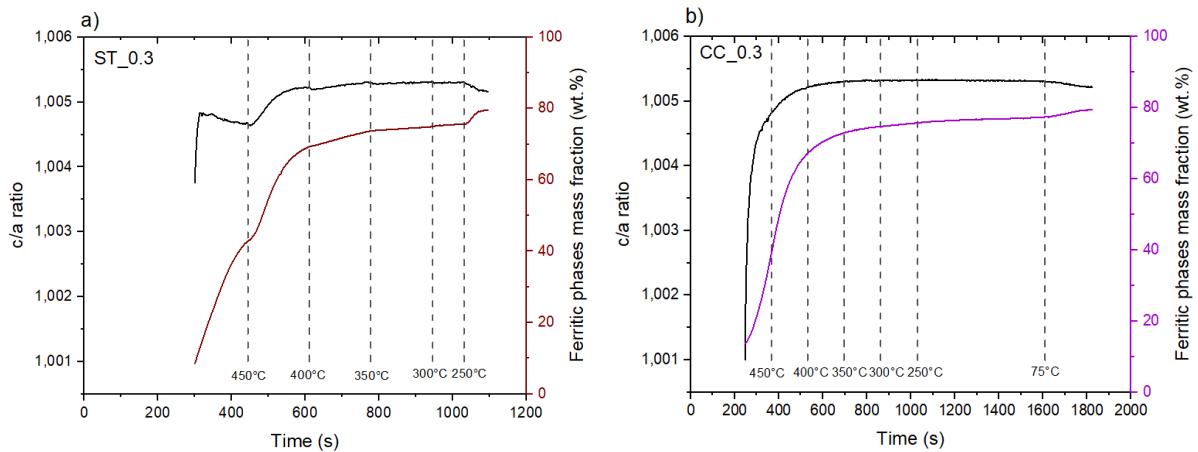
Figure. III. 25: Evolution of c/a ratio (black) and ferritic phases mass fraction as a function of time during a) experiment ST_0.3 (dark red) b) experiment CC_0.3 (purple).
