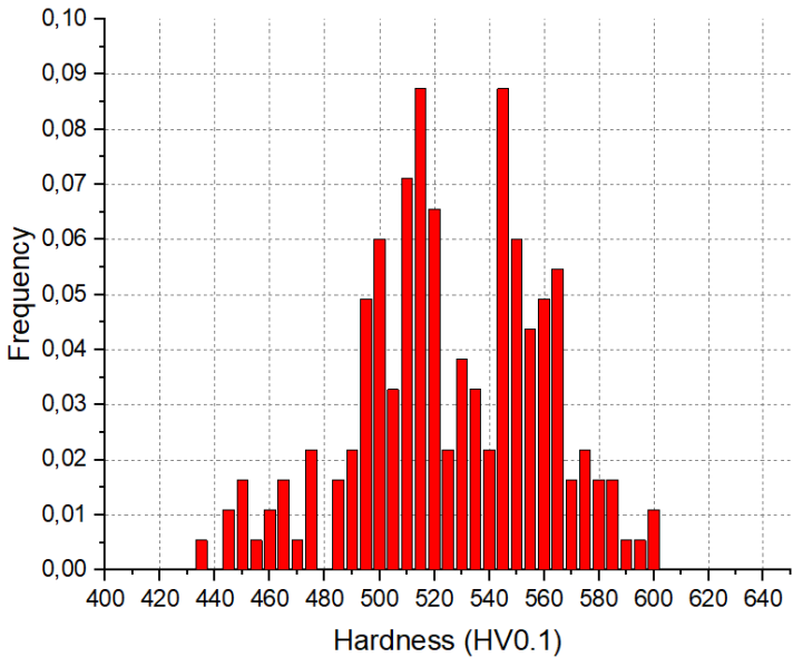
Figure. IV. 25: Distribution of hardness (HV0.1) for experiment ISO_475.
