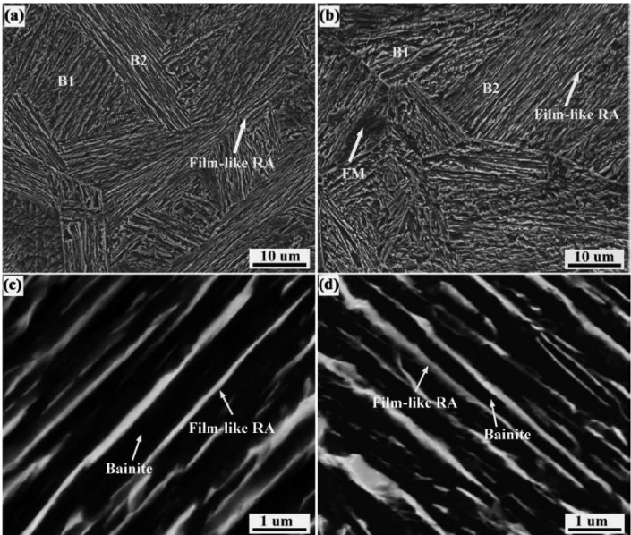
Figure. I. 27: SEM micrographs of the microstructures obtained after the two-step isothermal processes shown in Figure. I. 19: (a) and (c) sample 3 austempered at 430 °C for 2 min followed by 330 °C for 28 min; (b) and (d) sample 4 austempered 430 °C for 4 min followed by 330 °C for 26 min ; taken from [41].
