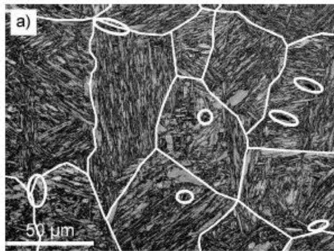
Figure. I. 10: Kikuchi Pattern Quality EBSD map (grey scale) of a 0.3C-2.5Mn-1.5Si-0.8Cr steel elaborated at M_s - 50^\circ\text{C} (austempering temperature). Prior austenitic grain boundaries have been highlighted (white lines) as well as some MA blocks (white circle), taken from [38].
