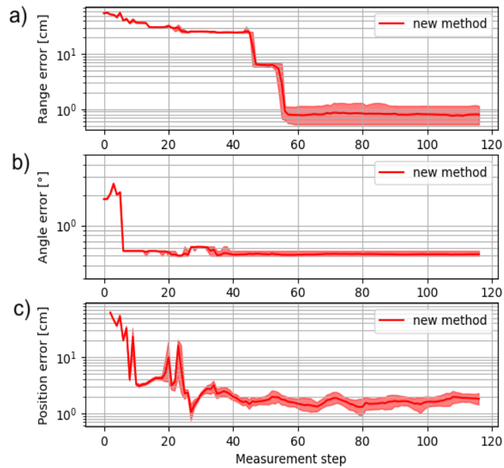
Figure 4.9: Localization and mapping results over 100 repetitions of a lawn-mower path on plate 2 for the new FastSLAM method. a) Average estimation errors on the range parameter of the lines. b) Average estimation error on the angle parameter. c) Average localization errors in the estimated plate frame. The 10% and 90% quantiles correspond to the upper and lower bounds of the colored areas. The scales along the y-axis are logarithmic.
