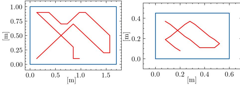
Figure 7.6: Simulated robot paths used for the experiments on the steel plate (left) and the aluminum plate (right). The path lengths ( i.e. the number of acquisition positions) are respectively 36 and 26.
