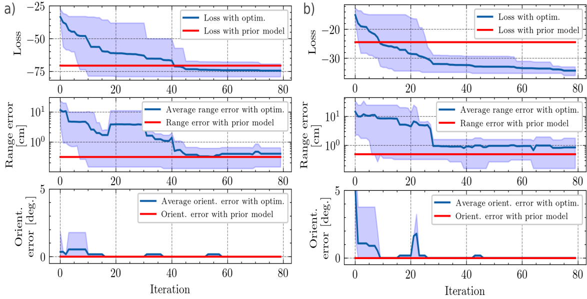
Figure 7.4: Evolution of the loss value and reconstruction errors for 10 repetitions of the optimization process with simulated annealing, and using the data from Scenario 1 (a) and Scenario 2 (b). The solid lines represent the mean values. The upper and lower bounds of the filled areas represent the minimum and maximum values respectively during each iteration. For comparison, the values achieved with the predetermined propagation model for each scenario are displayed as horizontal lines. The scale along the y-axis is logarithmic for the range error plots only.
