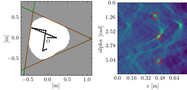
(a) 3 edges geometry
