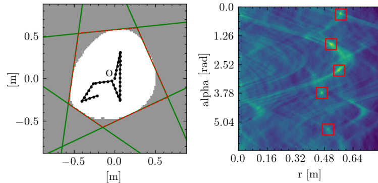
(c) 5 edges geometry.
