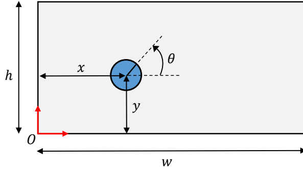
Figure 3.1: Illustration representing a robotic agent whose pose is \mathbf{x} = [x, y, \theta]^T on a rectangular metal plate of dimensions w \times h .
