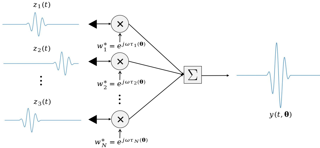
Figure 2.4: Illustration of delay-and-sum beamforming to achieve source localization. The filter weights \mathbf{w}(\boldsymbol{\theta}) apply delays to the input signals based on the distance between each antenna element and candidate position \boldsymbol{\theta} . The beamformer outputs the sum of the delayed signals which presents constructive interference when the candidate \boldsymbol{\theta} matches the true source location.
