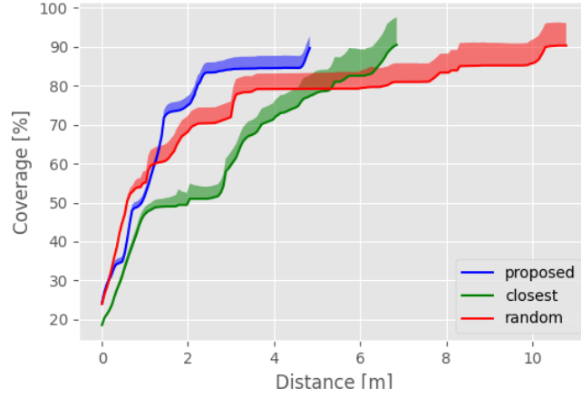
Figure 5.12: Evolution of the plate surface coverage for the three exploration strategies with respect to the traveled distance during the experiments. The solid lines represent the coverage mean value over 5 repetitions of each method, while the upper and lower bounds of the colored areas represent respectively the 90% and 10% quantiles.
