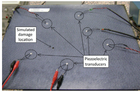
(a) Picture of the experimental setup.
