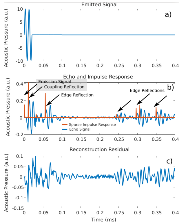
Figure 4.2: Illustration of the echo detection process. Panel a) shows the emitted signal. Panel b) shows the echo signal (blue trace) and the reconstructed impulse response (orange trace). Panel c) shows the reconstruction residual.
