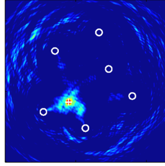
(b) Guided wave imaging results.
