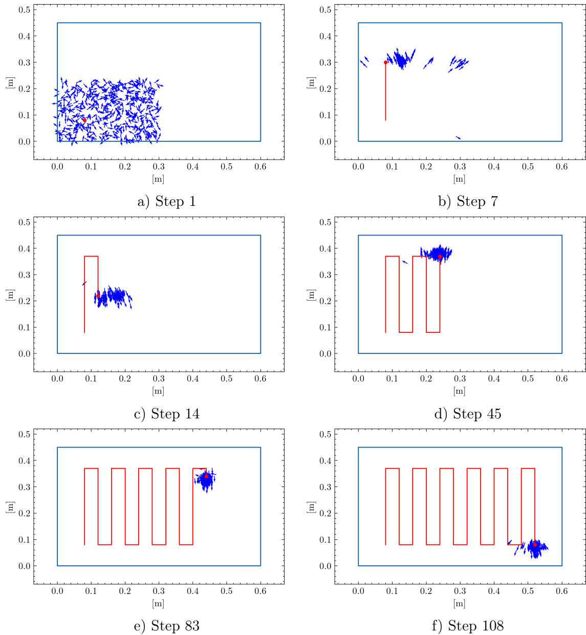
Figure 3.7: Qualitative localization results of the particle filter during measurement steps 1, 7, 14, 45, 83 and 108 of the simulated lawn mowing trajectory. The red dot represents the ground truth sensor position, the red line accounts for the true sensor trajectory. The blue rectangle represents the outline of the plate, and the arrows account for the particles' distribution.
