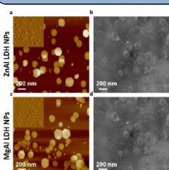
Fig. 2: SEM and STM images of ZnAl (a,b) and MgAl (c,d) LDH NPs.
