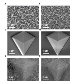
Fig. 6: SEM images of LDH films on silicon wafers and AFM tips. (a) ZnAl LDH film grown on Si wafer. (b) MgAl LDH film grown on Si wafer. (c) Bare AFM tip. (d) Aluminum-coated AFM tip. (e) ZnAl LDH-functionalized Al/M tip. (f) MgAl LDH-functionalized Al/M tip.
