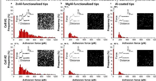
Fig. 7: Adhesion force histograms and adhesion force maps (areas, 400 \times 400 nm 2 ) obtained on the top of cells in using ZnAl-functionalized AFM tips (a) MgAl-functionalized AFM tips (b) Al-coated AFM tips (c). White/grey pixels correspond to adhesive events and black pixels correspond to non-adhesive events (scale 0-1000 pN).
