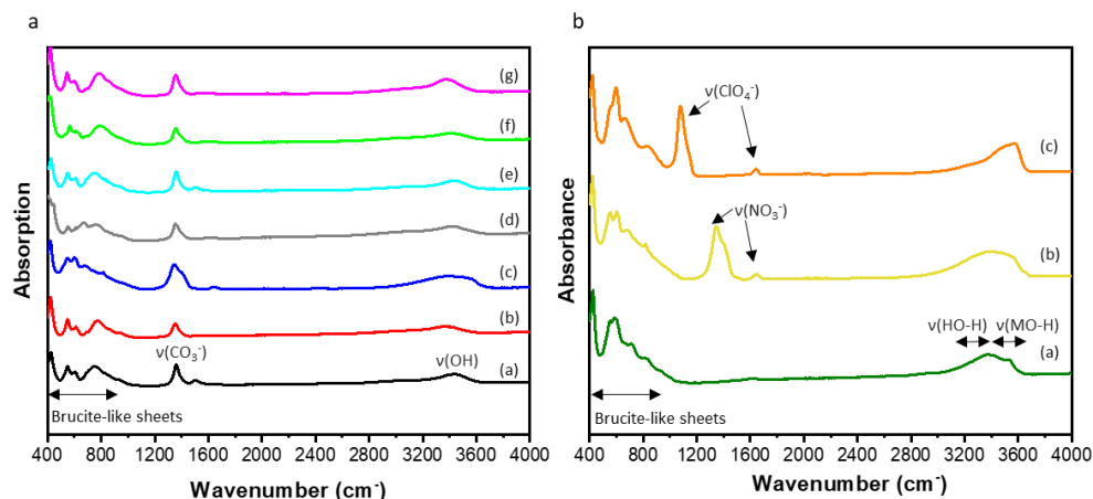
Figure 3. a) Infrared spectra of carbonate-intercalated LDHs: (a) Zn 2 Al:CO 3 -hyd, (b) Zn 2 Al:CO 3 -cop, (c) Zn 3 Al:CO 3 , (d) Mg 2 Al:CO 3 , (e) Cu 2 Al:CO 3 , (f) Ni 2 Al:CO 3 , (g) Co 2 Al:CO 3 . b) Infrared spectra of chloride-, nitrate- and perchlorate intercalated LDHs. (a) Zn 2 Al:Cl, (b) Zn 2 Al:NO 3 , (c) Zn 2 Al:ClO 4 .
