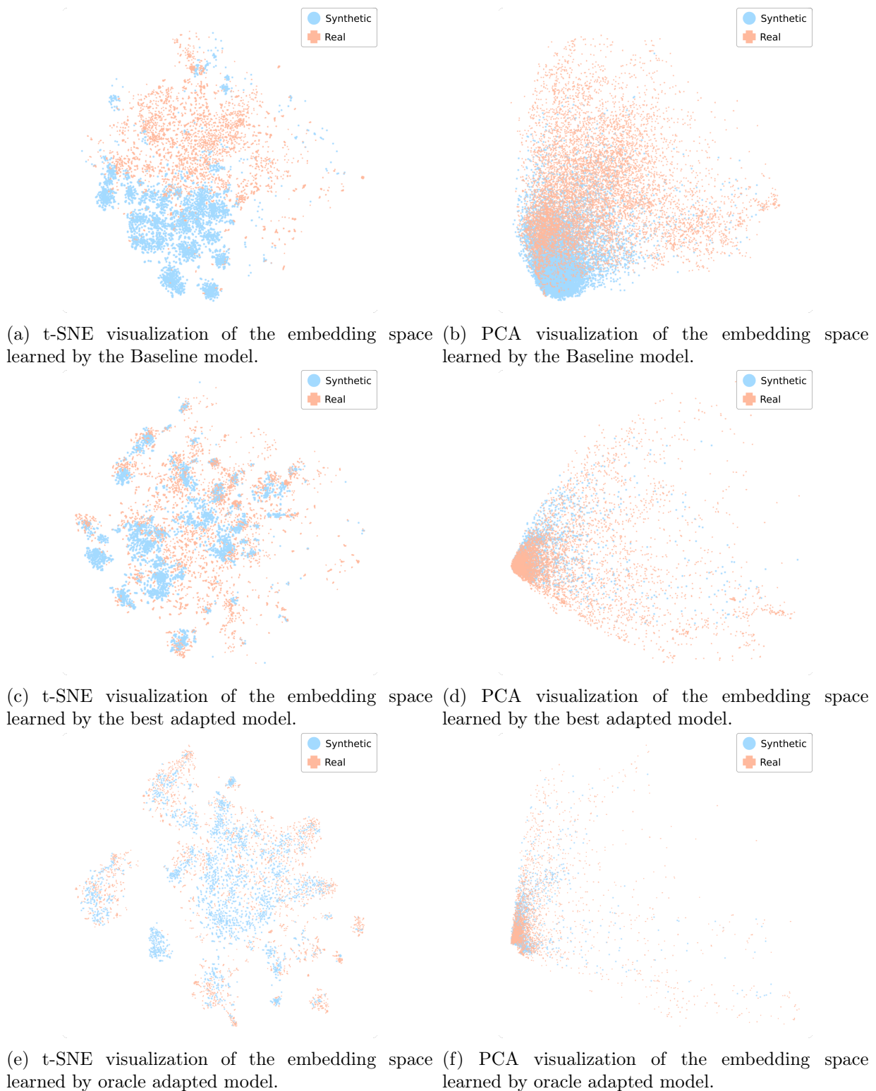
Figure 5.15: t-SNE (left column) and PCA (right column) visualizations of the distribution of learned embeddings by the Baseline model (top row), by the best model adapted using inactive frames only (middle row) and by the oracle model using inactive frames only and performing adaptation with ground-truth data (bottom row). In this setting, the performance of the best model is below the baseline model.
