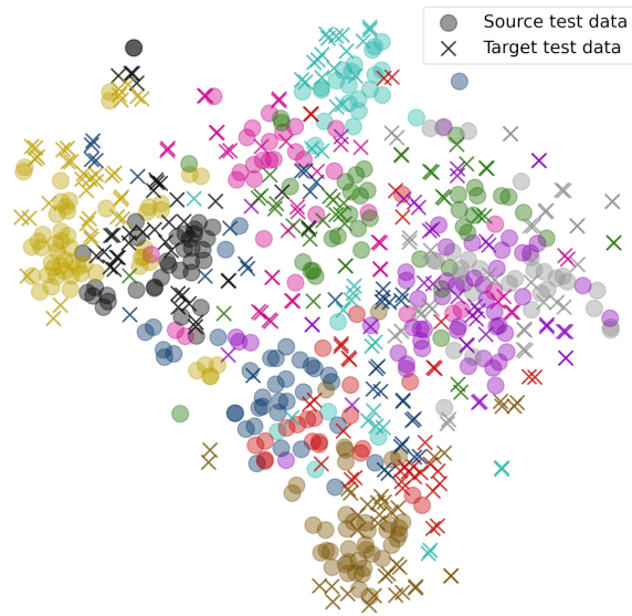
(b) Embedding space (device dep. setting).
