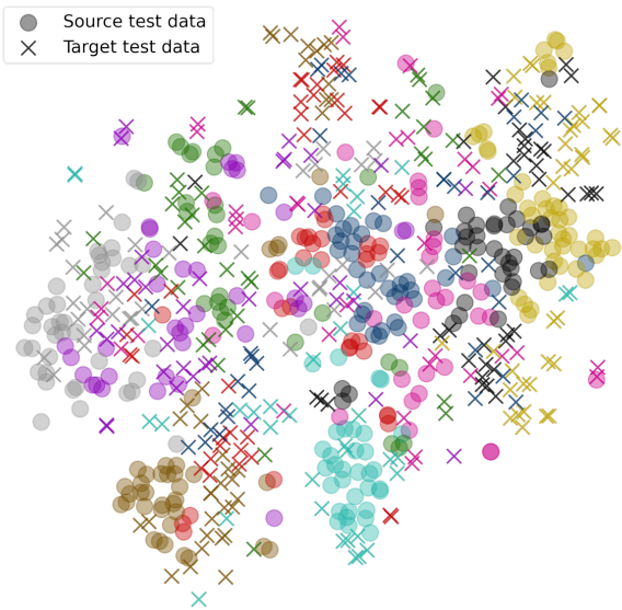
(a) Embedding space (device indep. setting).
