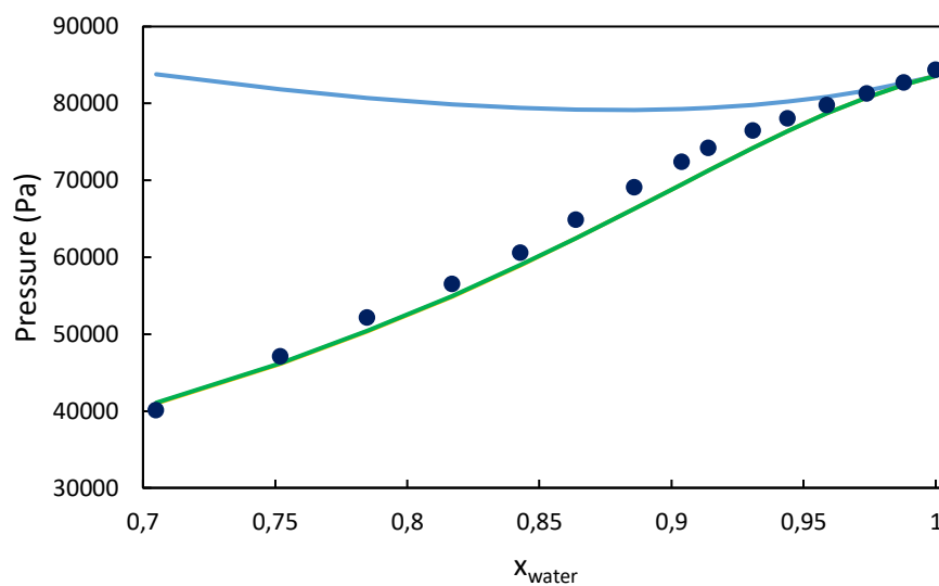
Figure 3.2. Isothermal vapour pressure versus mole fraction of water for the system {1-Methyl-1-pentylpyrrolidinium bromide + Water} at 368.15K, ● experimental data [68], — COSMO-SAC (2010) model, — COSMO-SAC (+OH-Br) model, — COSMO-SAC (+OH-ClBr) model (the two +OH-X models coincide)
