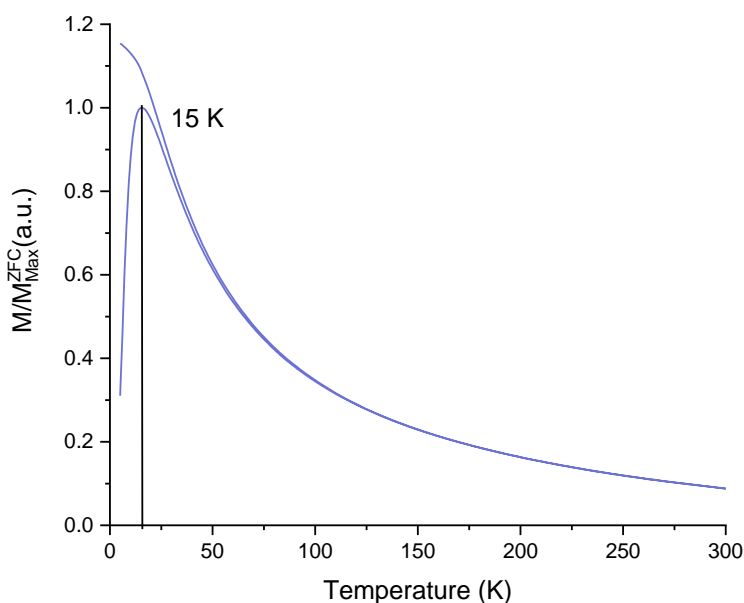
Figure 7: ZFC-FC curve of \text{NP}_{\text{SMW}}@\text{Cit} with a T_B = 15\text{K} .
