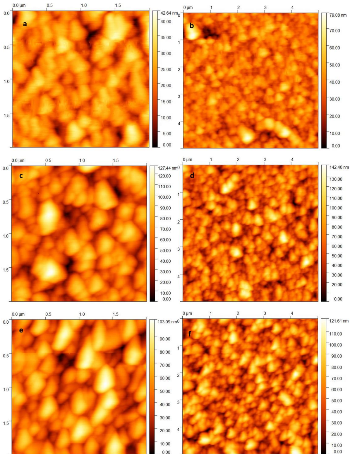
Figure II. 8. AFM topography images of (a-b) commercial and (c-d-e-f) sprayed FTO samples. the carrier gas flow for the sprayed samples is 9.05 \text{l}\cdot\text{min}^{-1} and 6.22 \text{l}\cdot\text{min}^{-1} respectively for (c-d) and (e-f).
