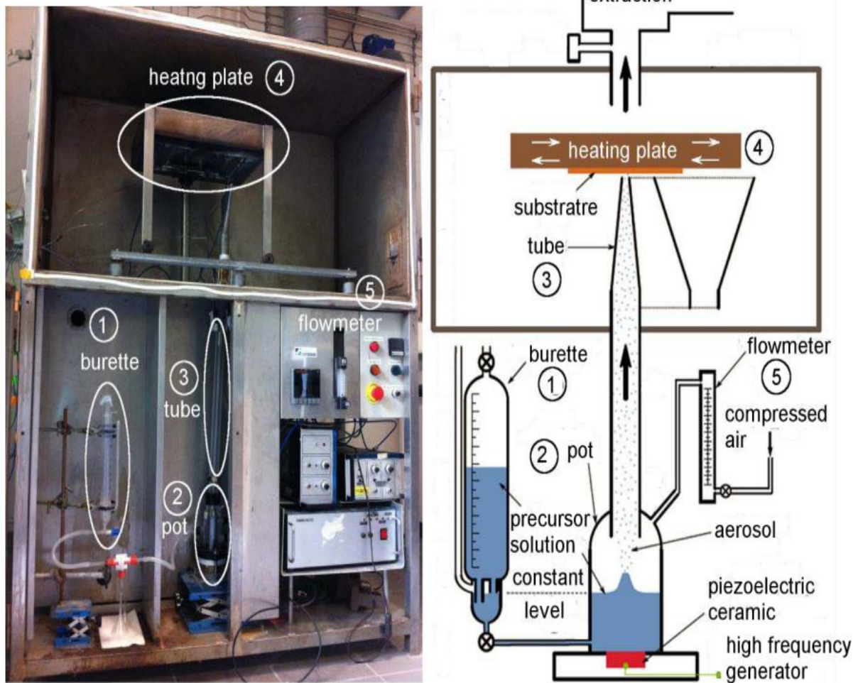
Figure II. 7. The setup of ultrasonic spray pyrolysis together with its schematics drawn for clarification at LMGP laboratory. 152
