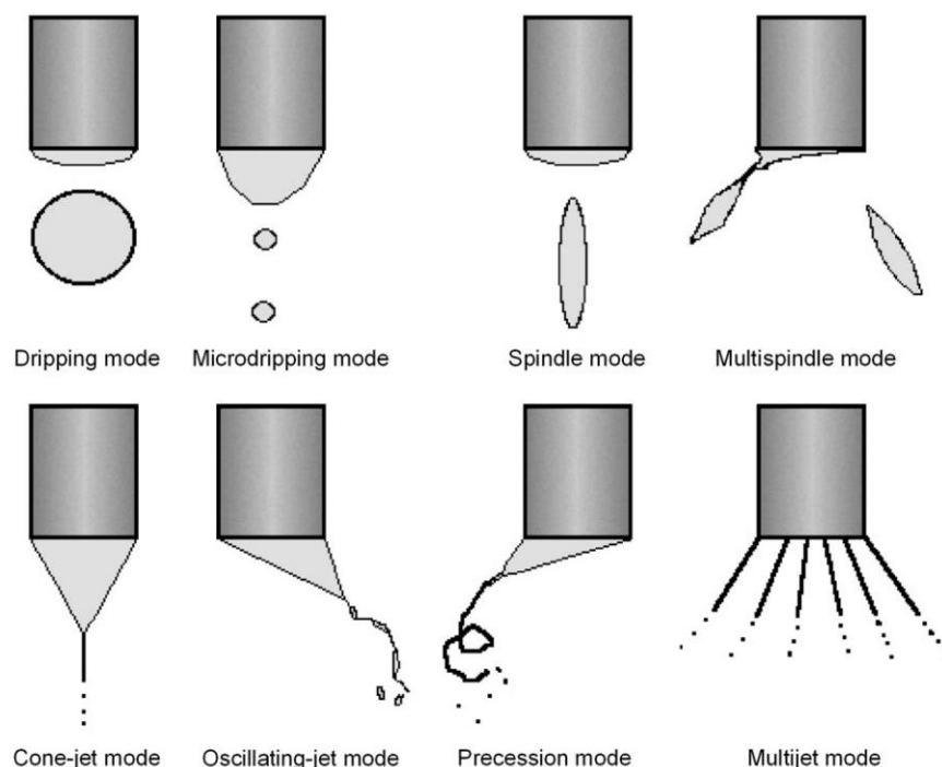
Figure III. 4. Scheme of different electrospay jet modes. 211
