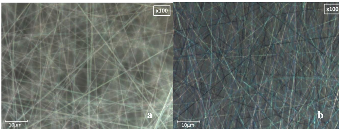
Figure III. 6. Microscopic images of Zinc Acetate fibers for a deposition time of 35 min; (a) before annealing with magnification of \times 100 ; (b) after annealing at 450^{\circ}\text{C} with magnification \times 100 .
