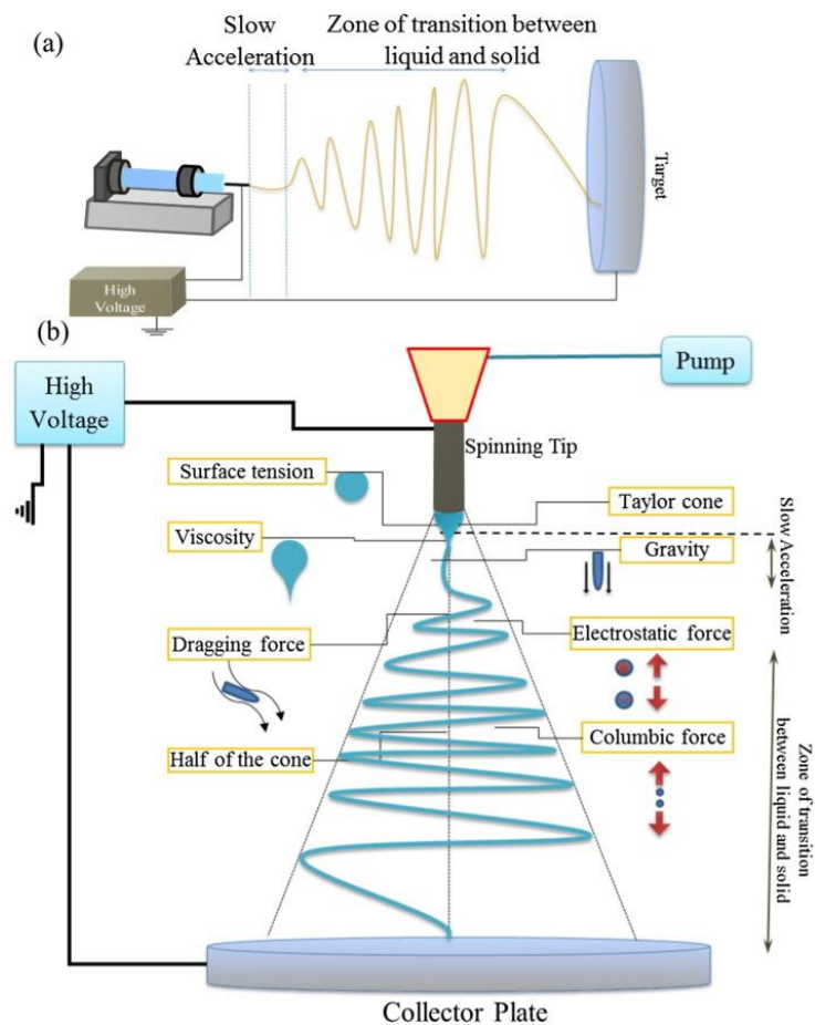
Figure III. 2. Typical electrospinning setup (a) horizontal, (b) vertical. (b) schematic diagram showing the electrospinning process with Taylor cone formation. 207
