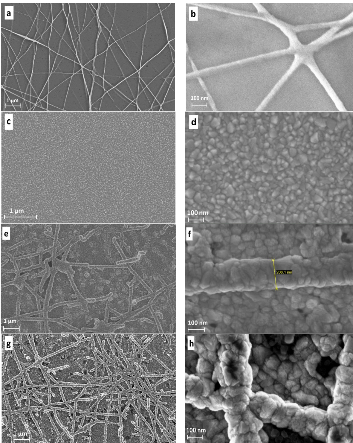
Figure III. 14. SEM images of FTO_ZnO nanocomposites with ZnO nanofibers deposited for: (a)-(b) 15min; (c)-(d) FTOstd reference sample; (e)-(f) 25 min and (g)-(h) 35 min.
