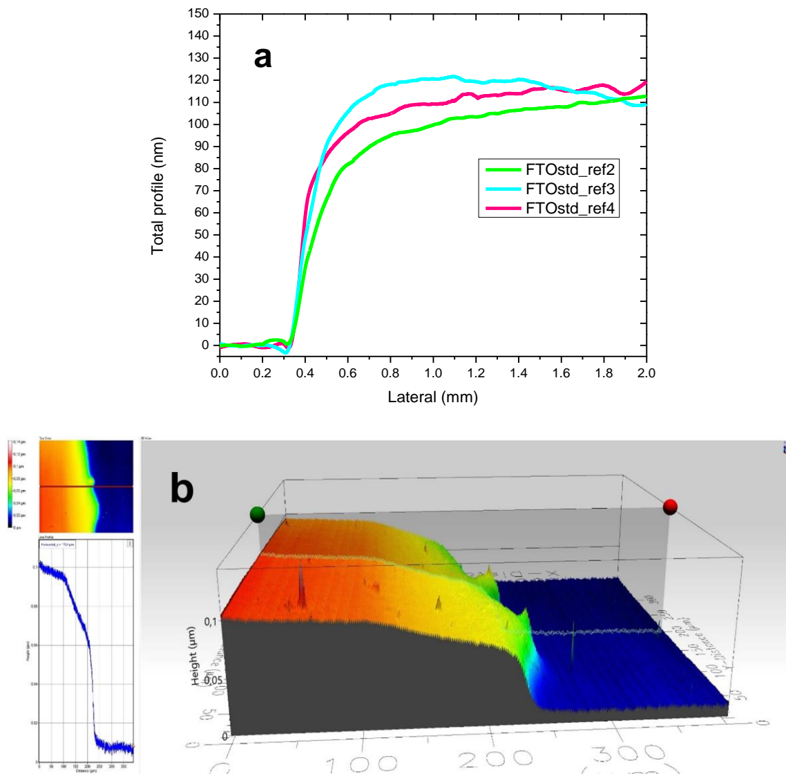
Figure III. 13. (a) Graph showing the thickness variation of FTOstd thin films with different deposition time. (b) Optical profilometer 3D profile of FTOstd_ref2 sample edge showing a thickness of 100nm.
