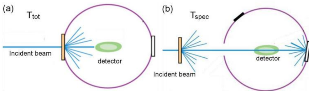
Figure III. 16. Schematic representation of the geometry for measuring (a) total transmittance ( T_{tot} ), (b) specular transmittance ( T_{spec} ). 152
