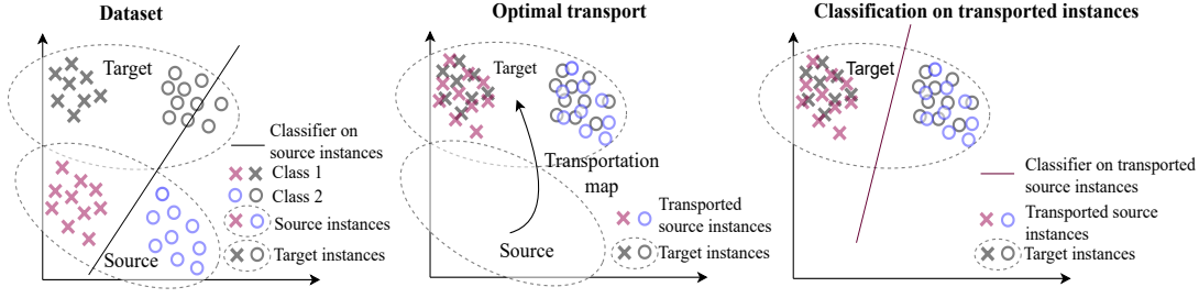
Figure 7.2: Illustration of the method proposed by Courty et al. (2017b) . The source and target domain datasets are presented on the left. A classifier trained on the source domain does not fit the target domain data. The source instances are transported onto the target domain by computing a transportation map in the center, usually with a non-linear transformation. The classifier in the target domain is estimated using the transported source instances.
